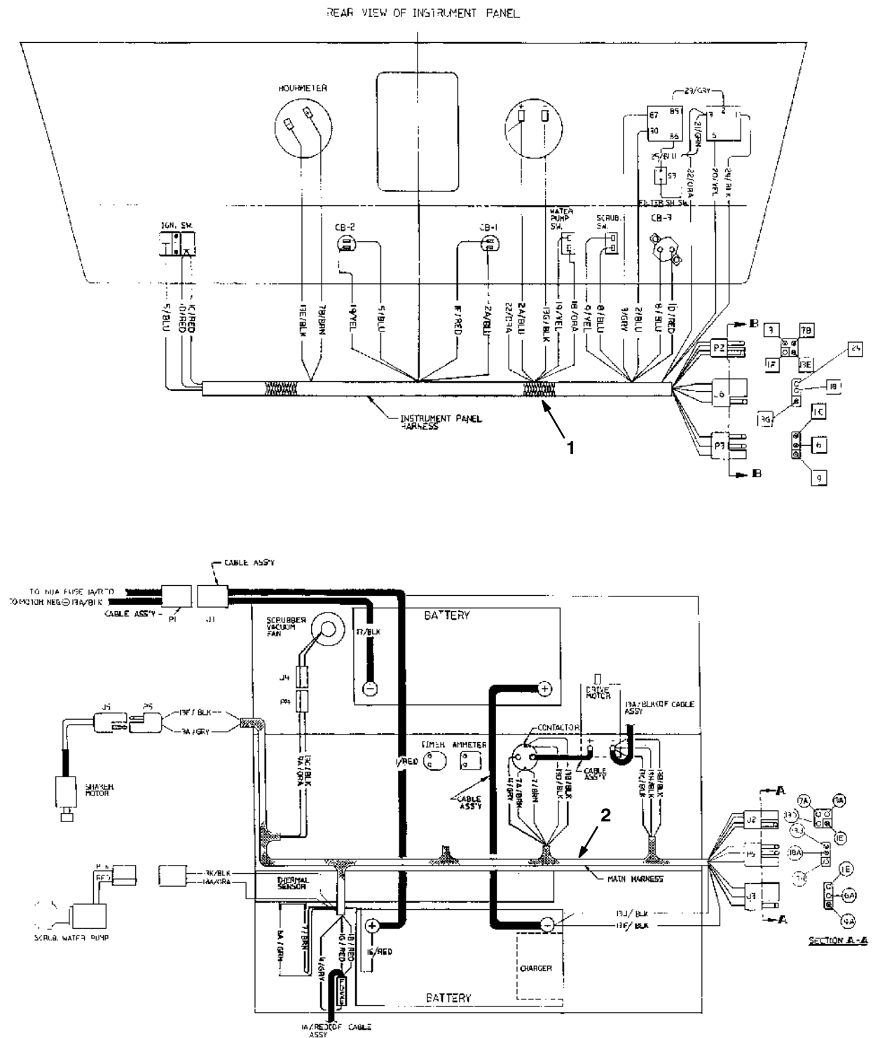
Fig. 19 – Wire Harnesses Group
