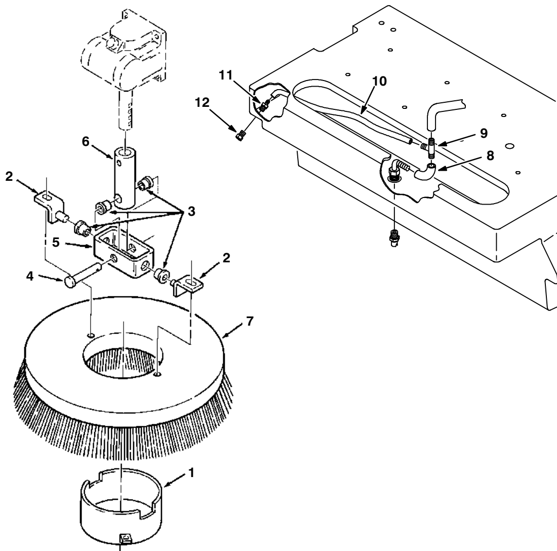
Fig. 2 – Side Scrub Brush Kit
