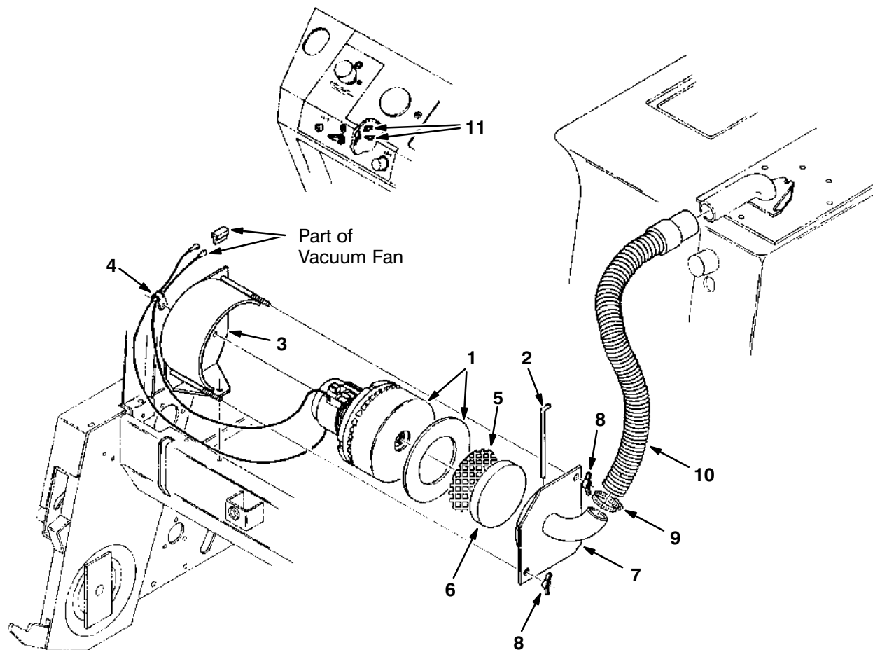
Fig. 13 – Scrub Vacuum Fan Group
