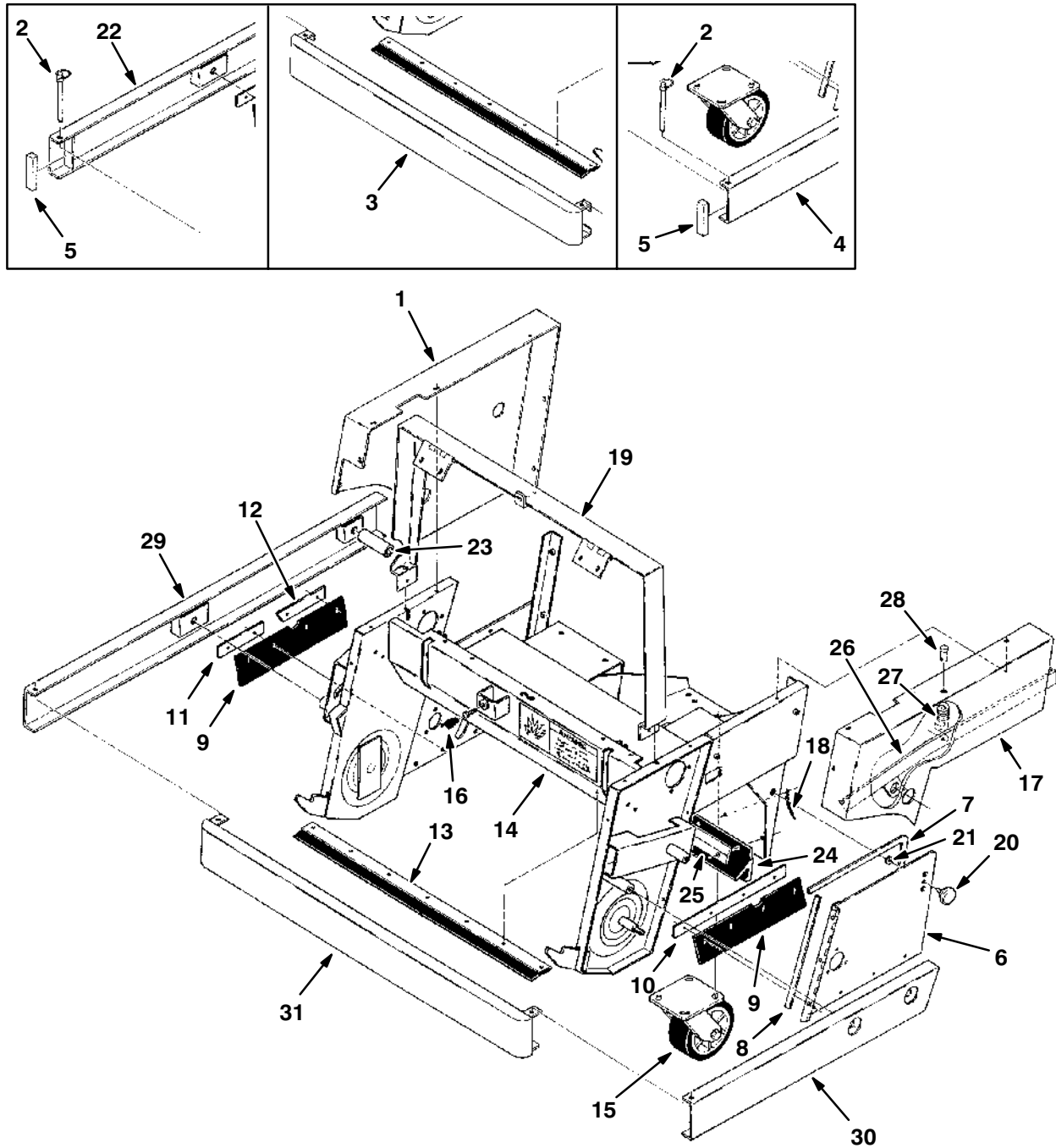
Fig. 3 – Main Frame Group
