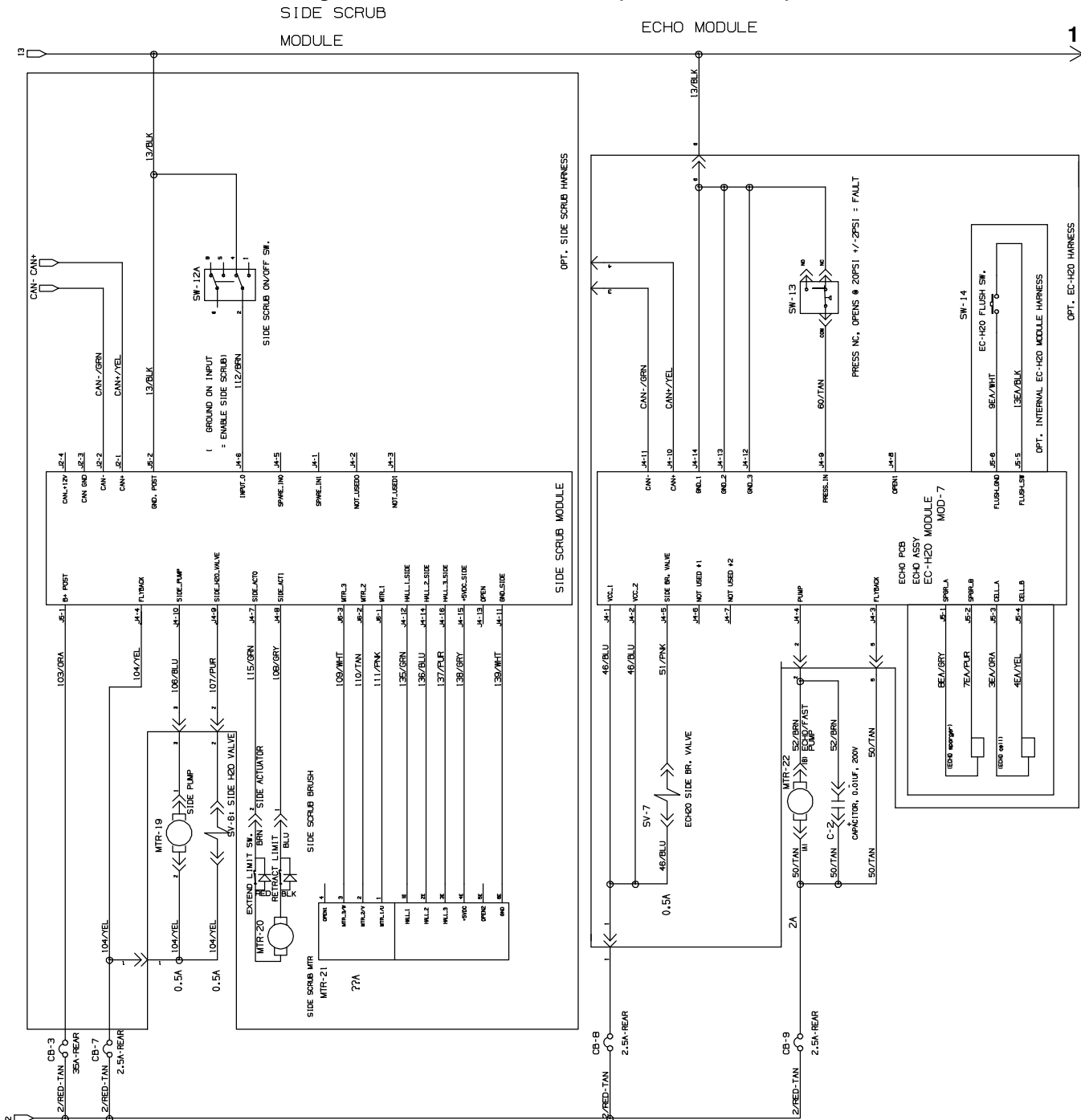
Fig. 51 – Electrical Schematic (000000-010999)
