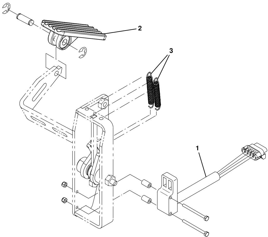
Fig. 2 – Accelerator and Brake Pedal Assembly Breakdown, 1209411
