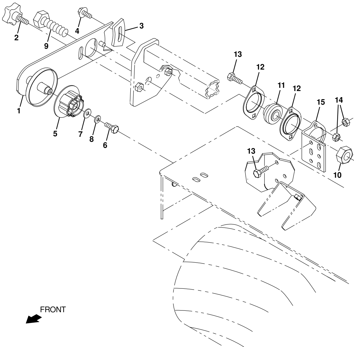
Fig. 43 – Direct Throw Main Brush Idler Group (011000– )
