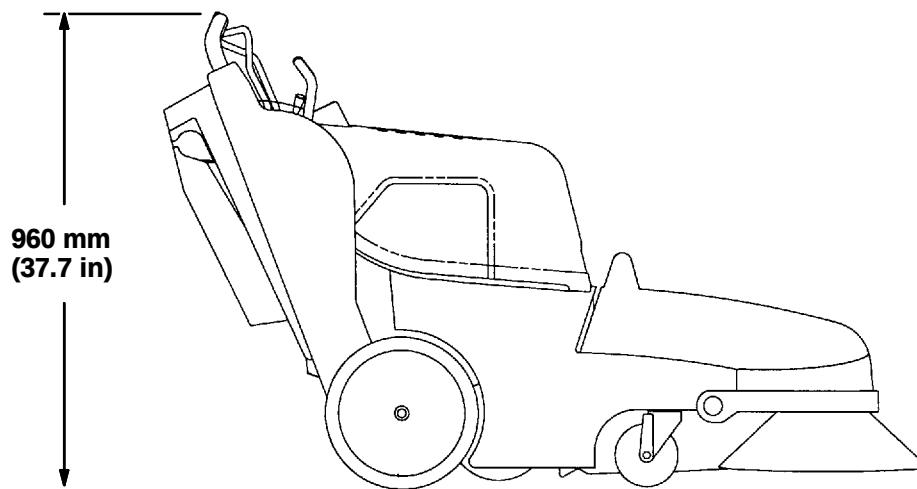
MACHINE DIMENSIONS
