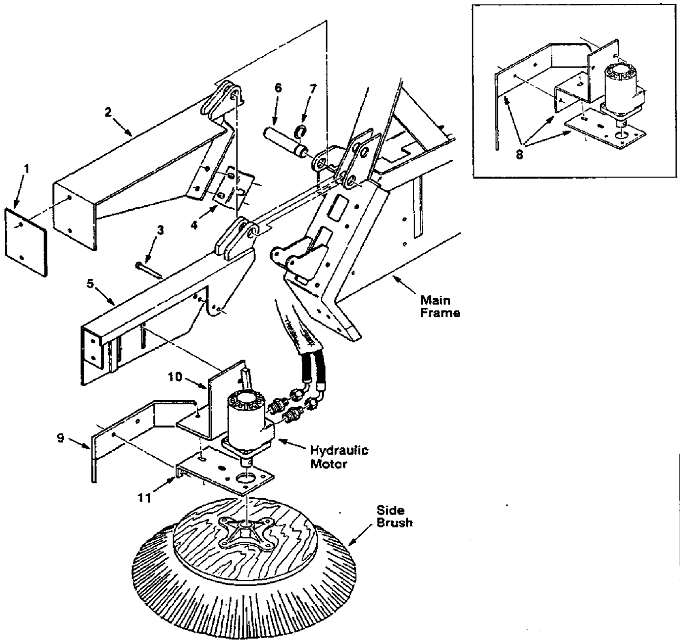
Fig. 8 - Side Brush Group, SE Multi-Level Dump
