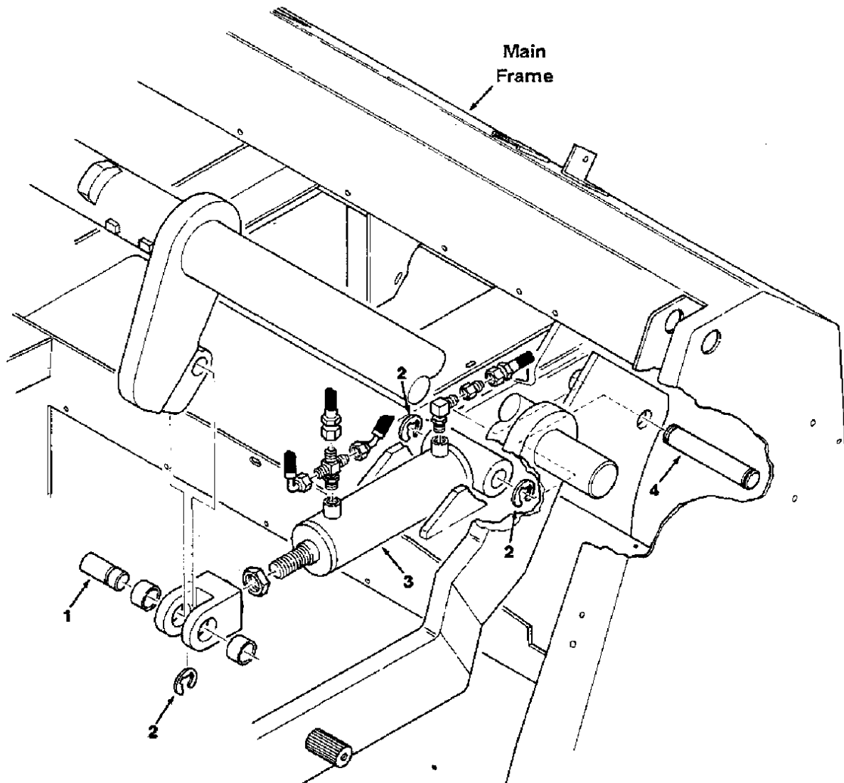
Fig. 6 - Hydraulic Lift Cylinder Group; SE Multi-Level Dump
