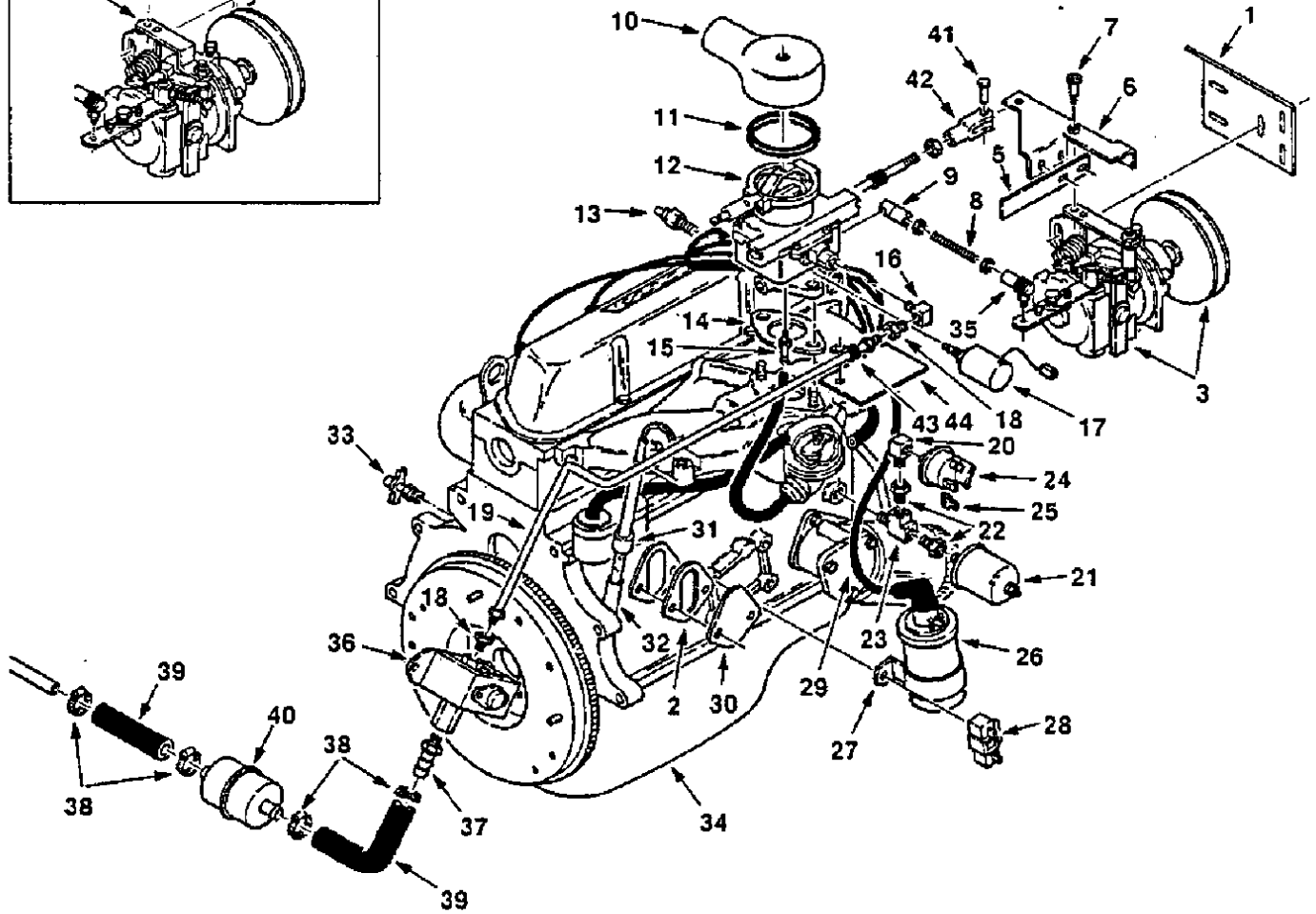
Fig. 27 - Engine Group
