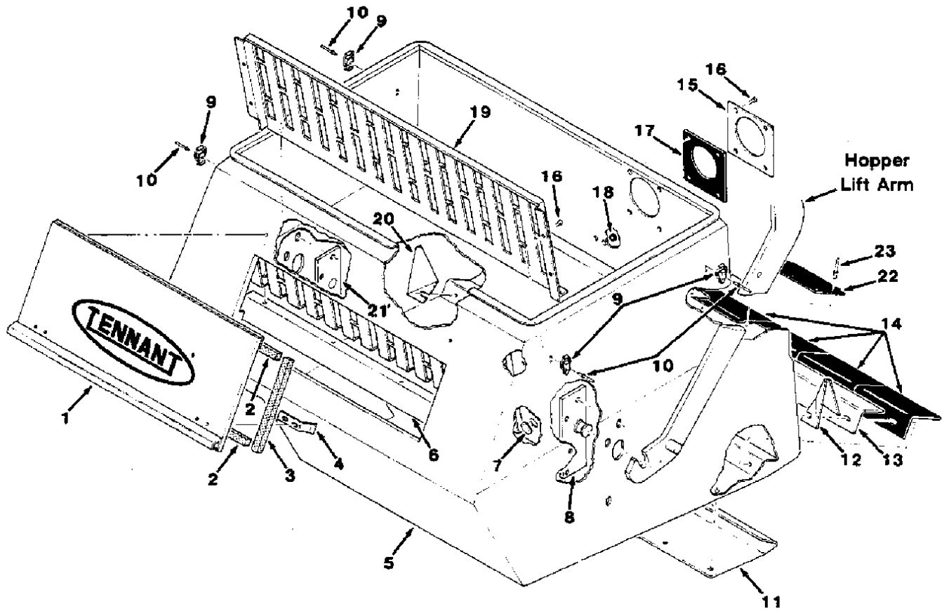
Fig. 6 - Hopper Group
