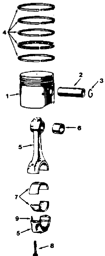
FIG. 5 - PISTON AND CONNECTING ROD GROUP
