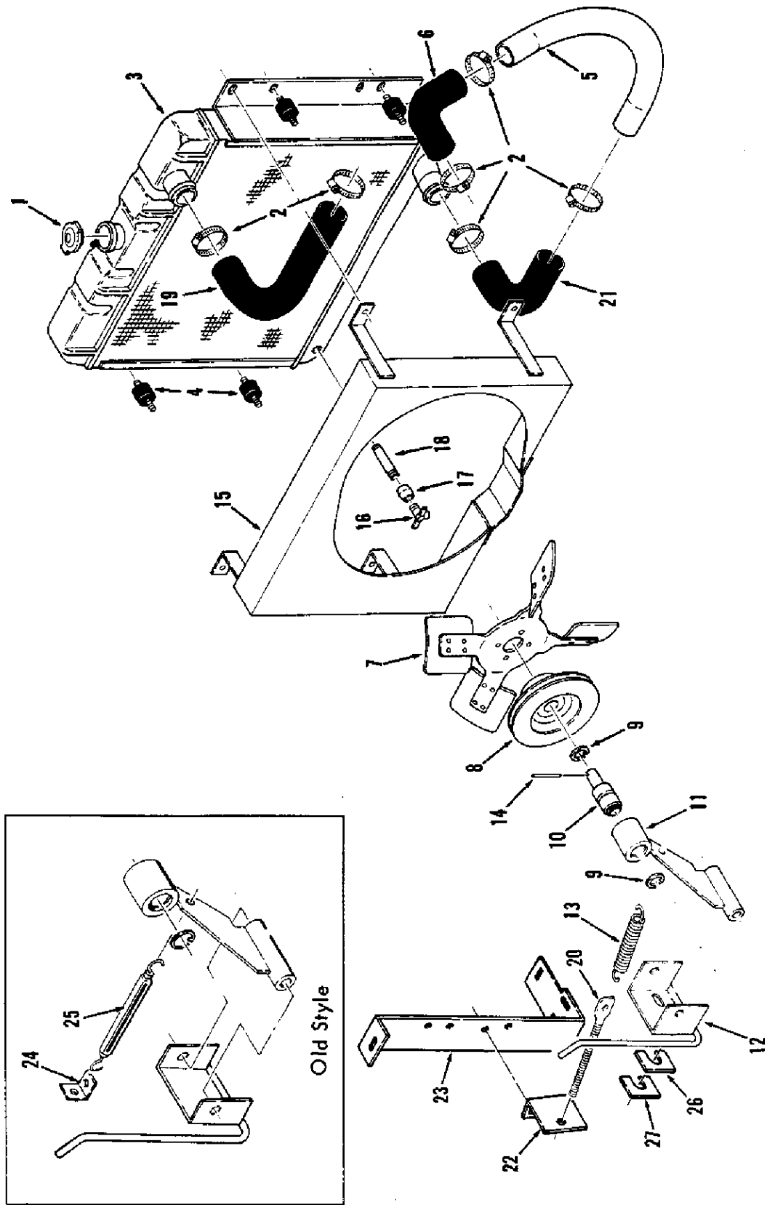
Fig. 12 - COOLING SYSTEM
