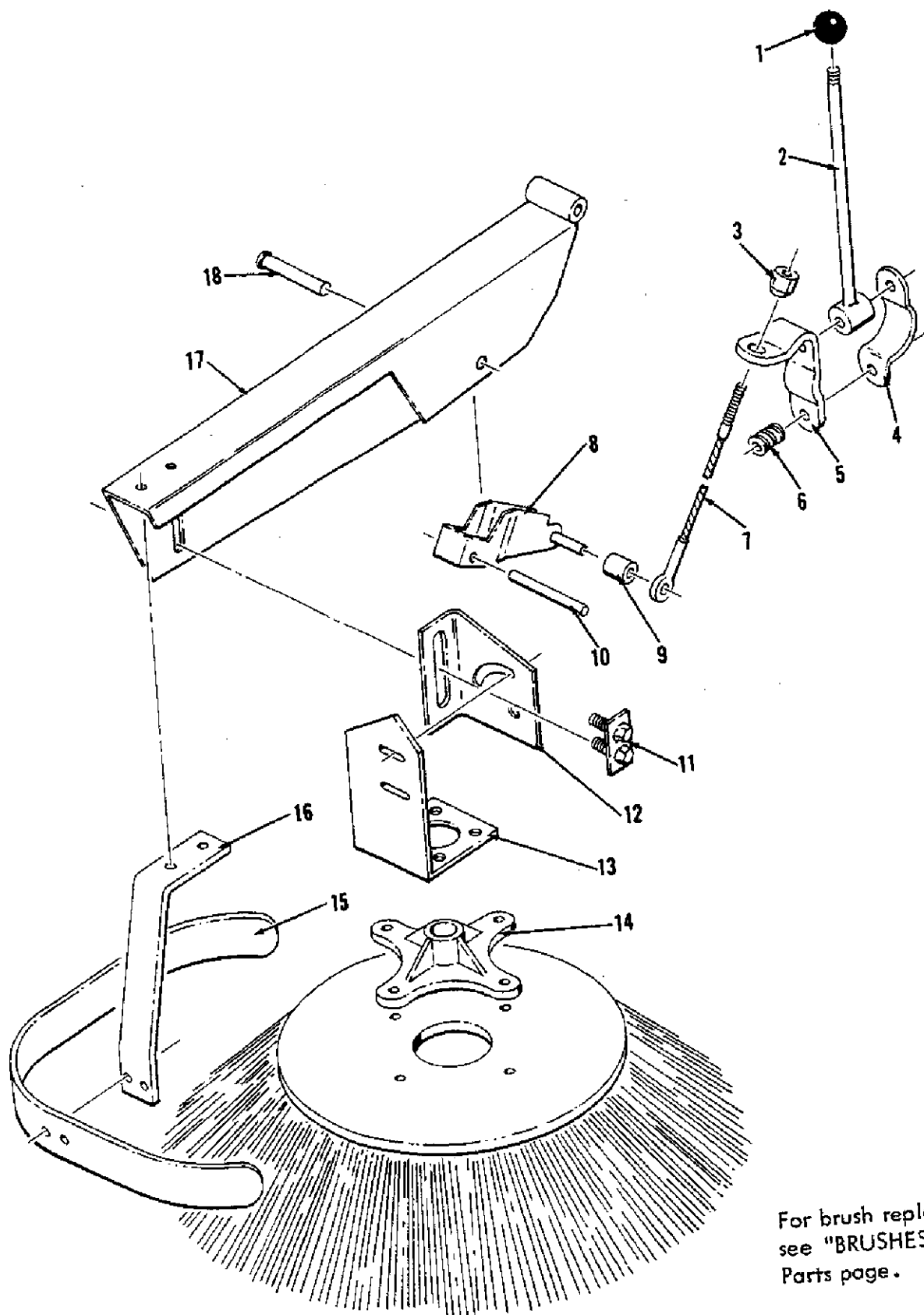
Fig. 15 - SIDE BRUSH SUPPORT & DRIVE 26
