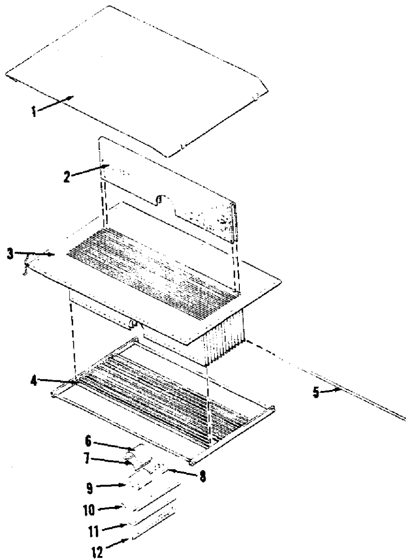
Fig. 6 - FILTER SYSTEM
