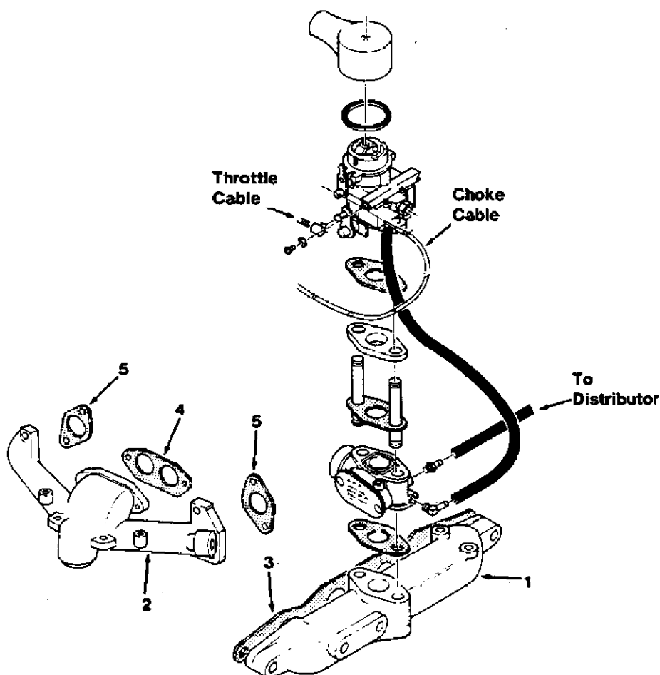
FIG. 8 - INTAKE, EXHAUST MANIFOLD, AND CARBURETOR GROUP
