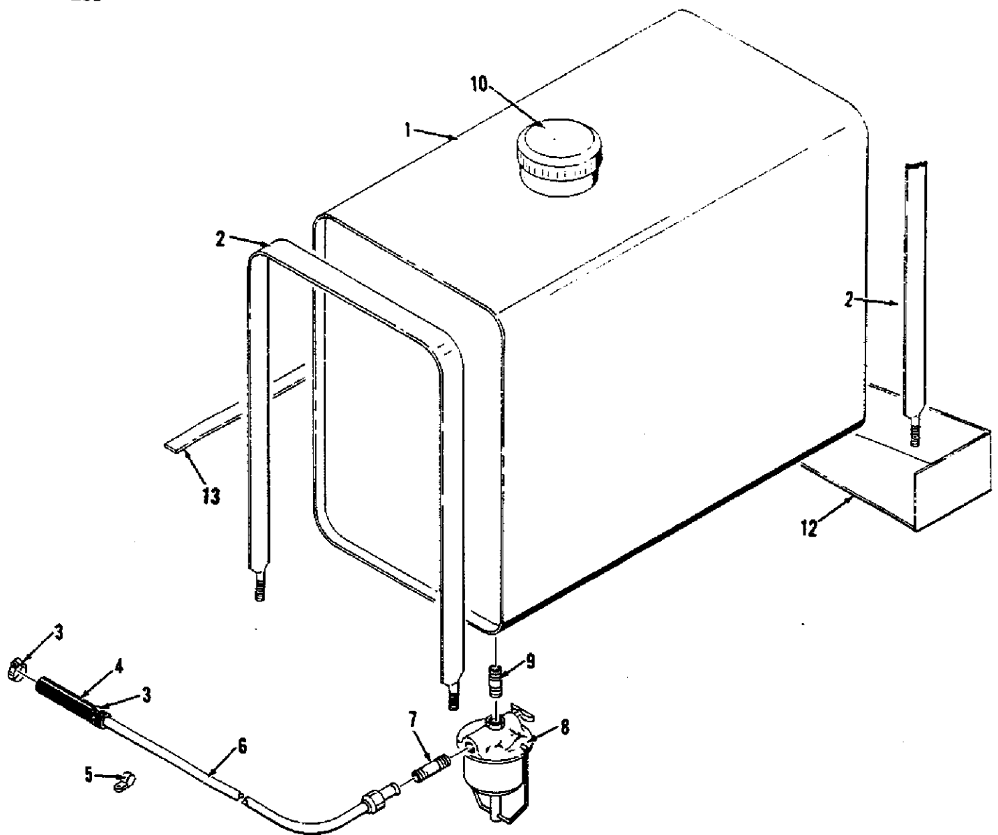
FIG. 10 - GASOLINE TANK &amp; FILTER
