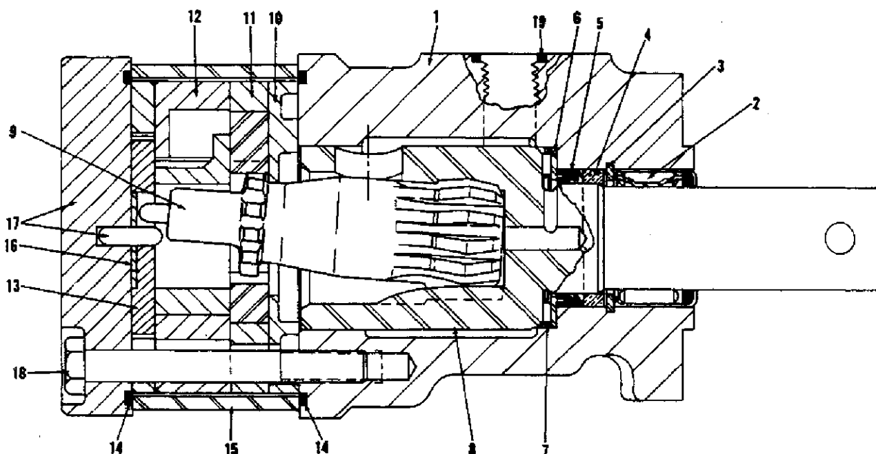
FIG. 7 - SIDE BRUSH MOTOR 47542
