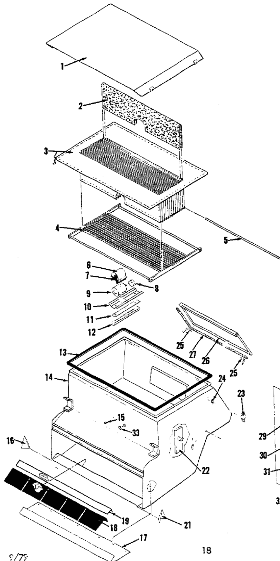
Fig. 9 FILTER SYSTEM
