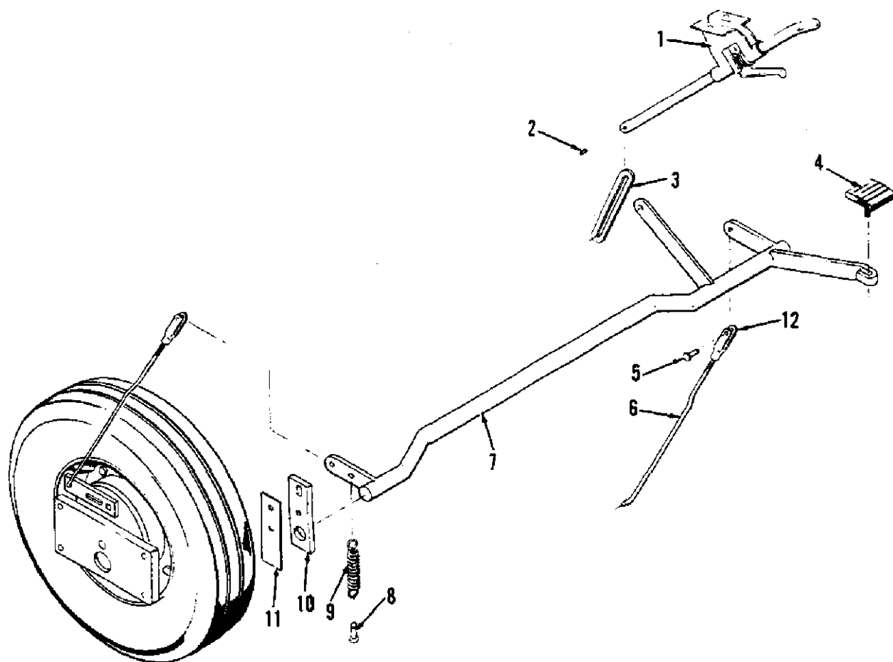
Fig. 17 - HANDBRAKE & FOOT BRAKE ASSEMBLY
