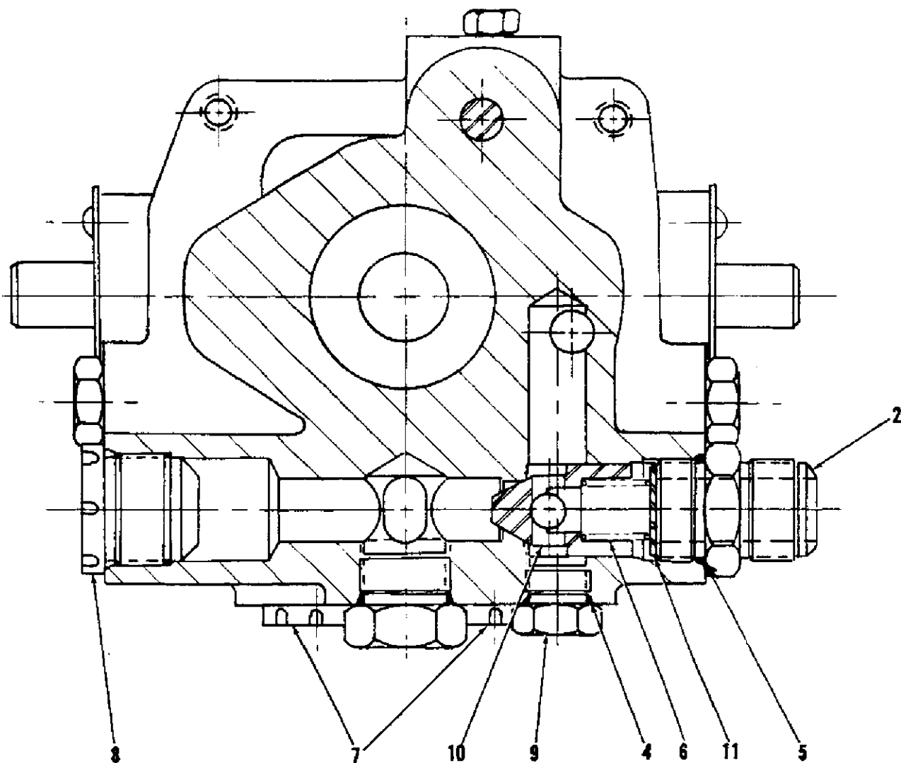
FIG. 3 - VICKERS TANDEM PUMPS NO. 47925 & 47861
