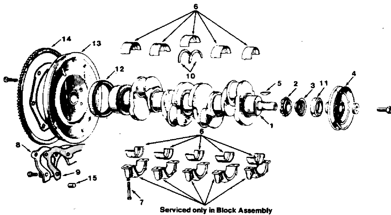
FIG. 2 - CRANKSHAFT GROUP
