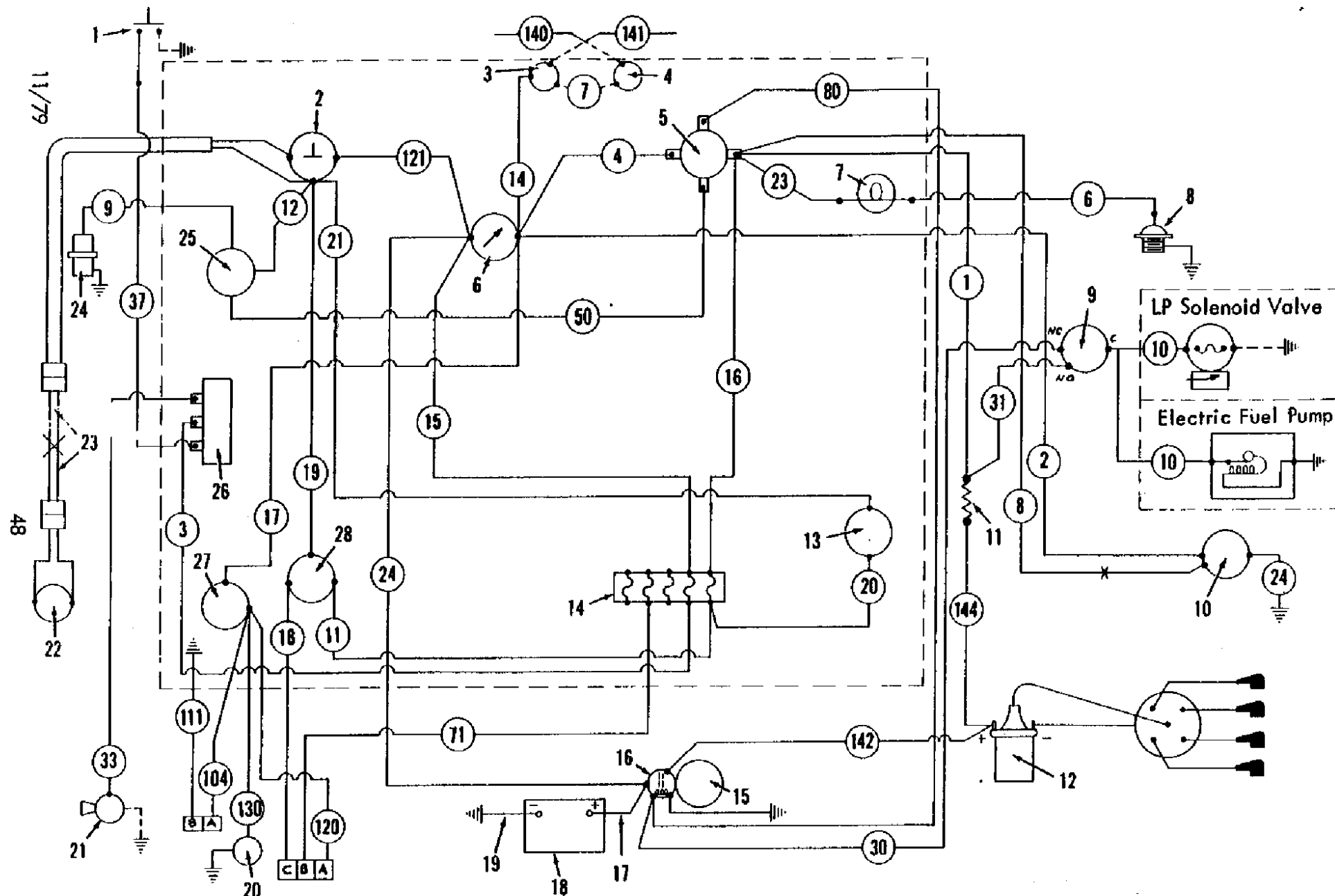
FIG. 24 - MODEL 265 ELECTRICAL SYSTEM (NOTE: Circled numbers are wire numbers. Plain numbers and arrows refer to Electrical System Parts List).
