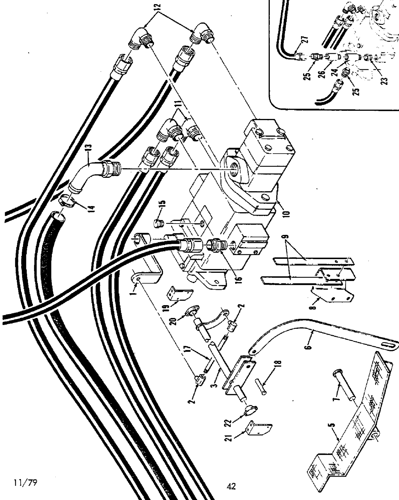
Fig. 21 - PUMP & CONTROL PARTS GROUP
