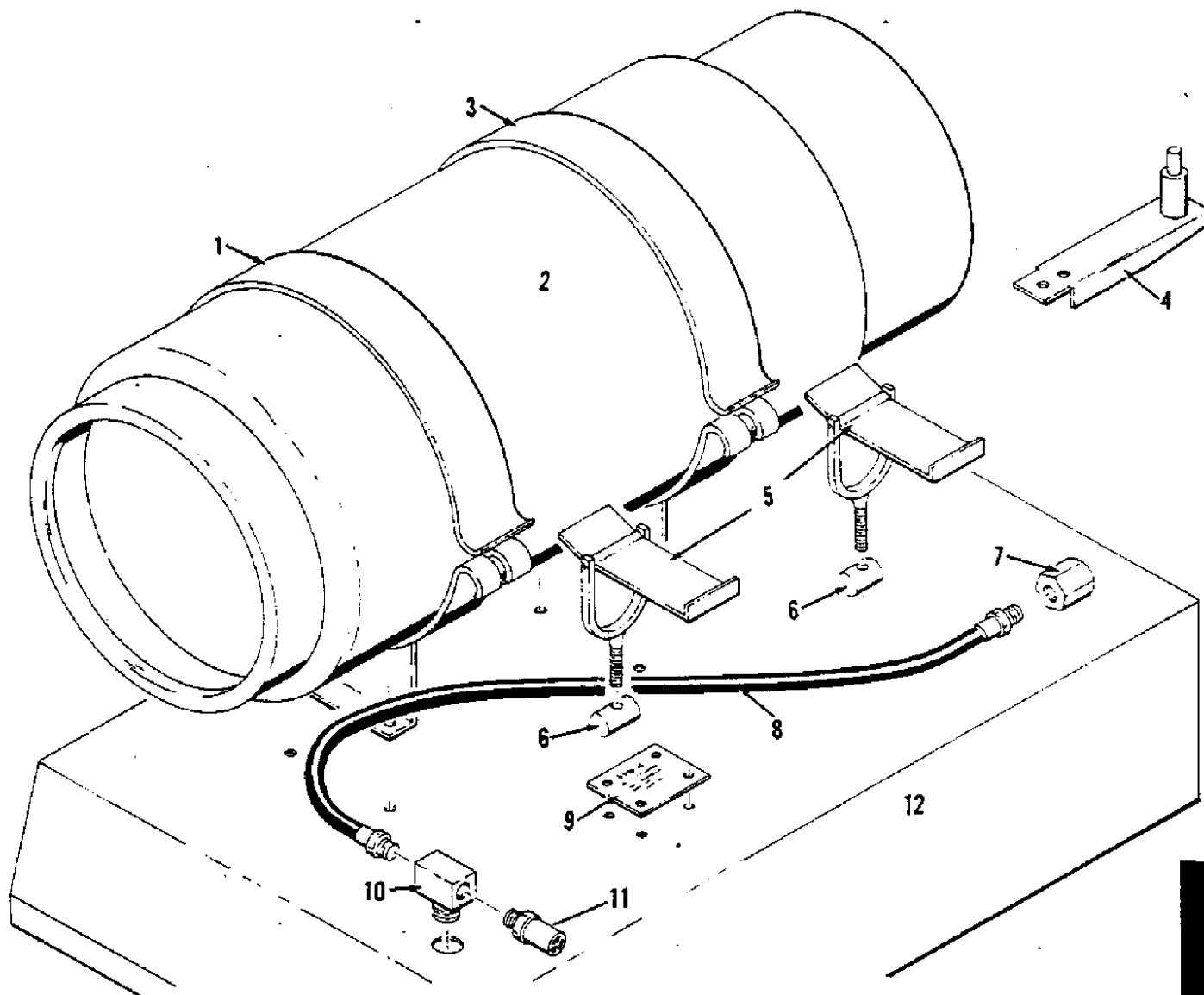
LP COMPONENTS - TANK AND COVER GROUP
