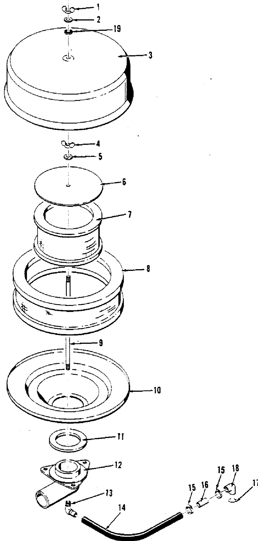
Fig. 4 - AIR CLEANER AND RELATED PARTS 8
