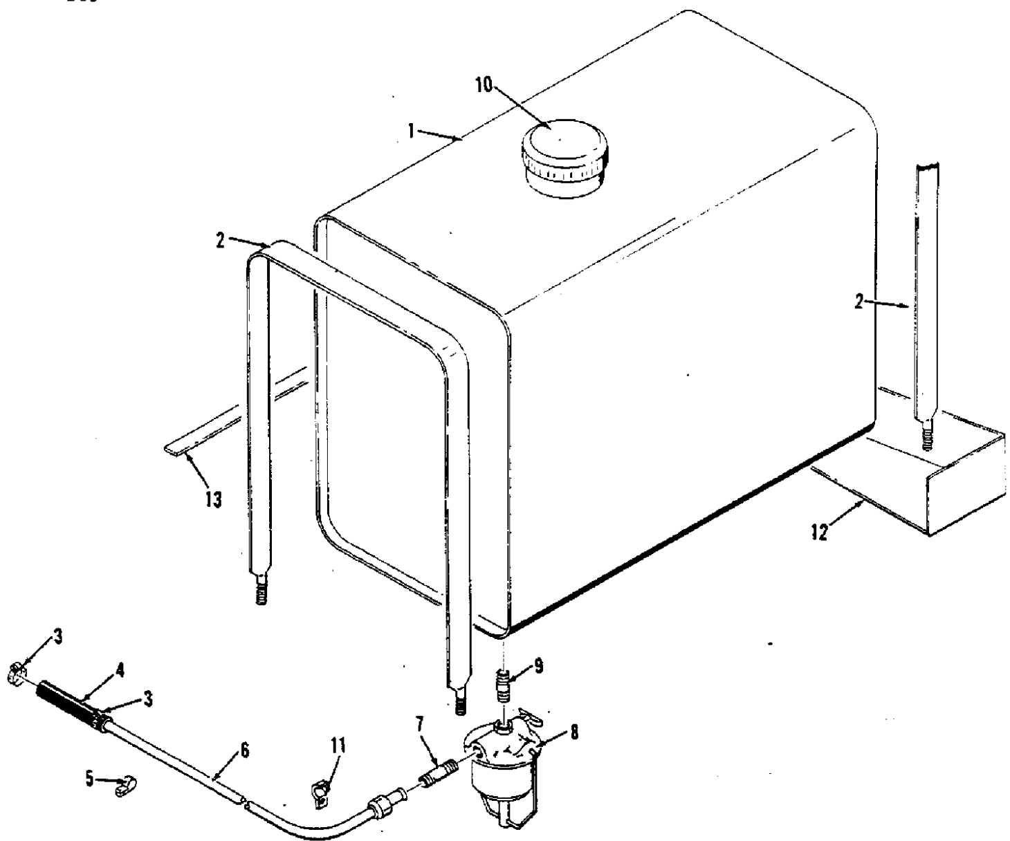
FIG. 10 - GASOLINE TANK &amp; FILTER
