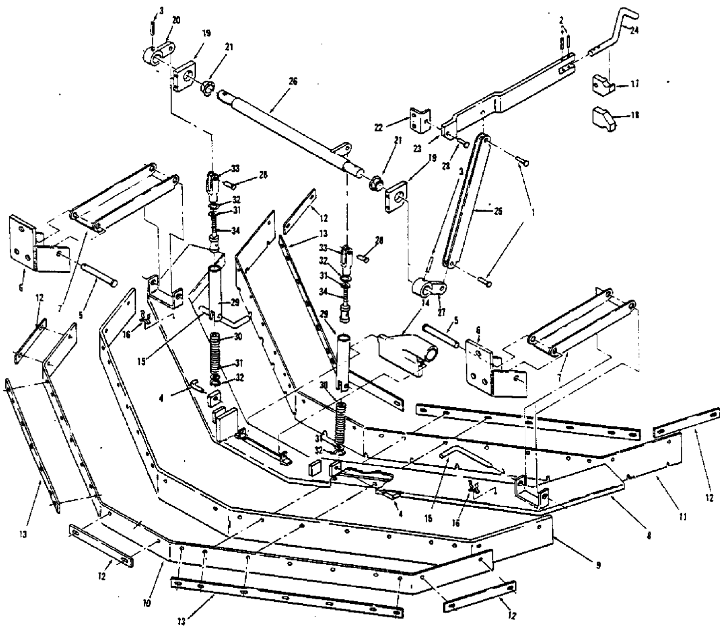
Fig. 4 - REAR SQUEEGEE
