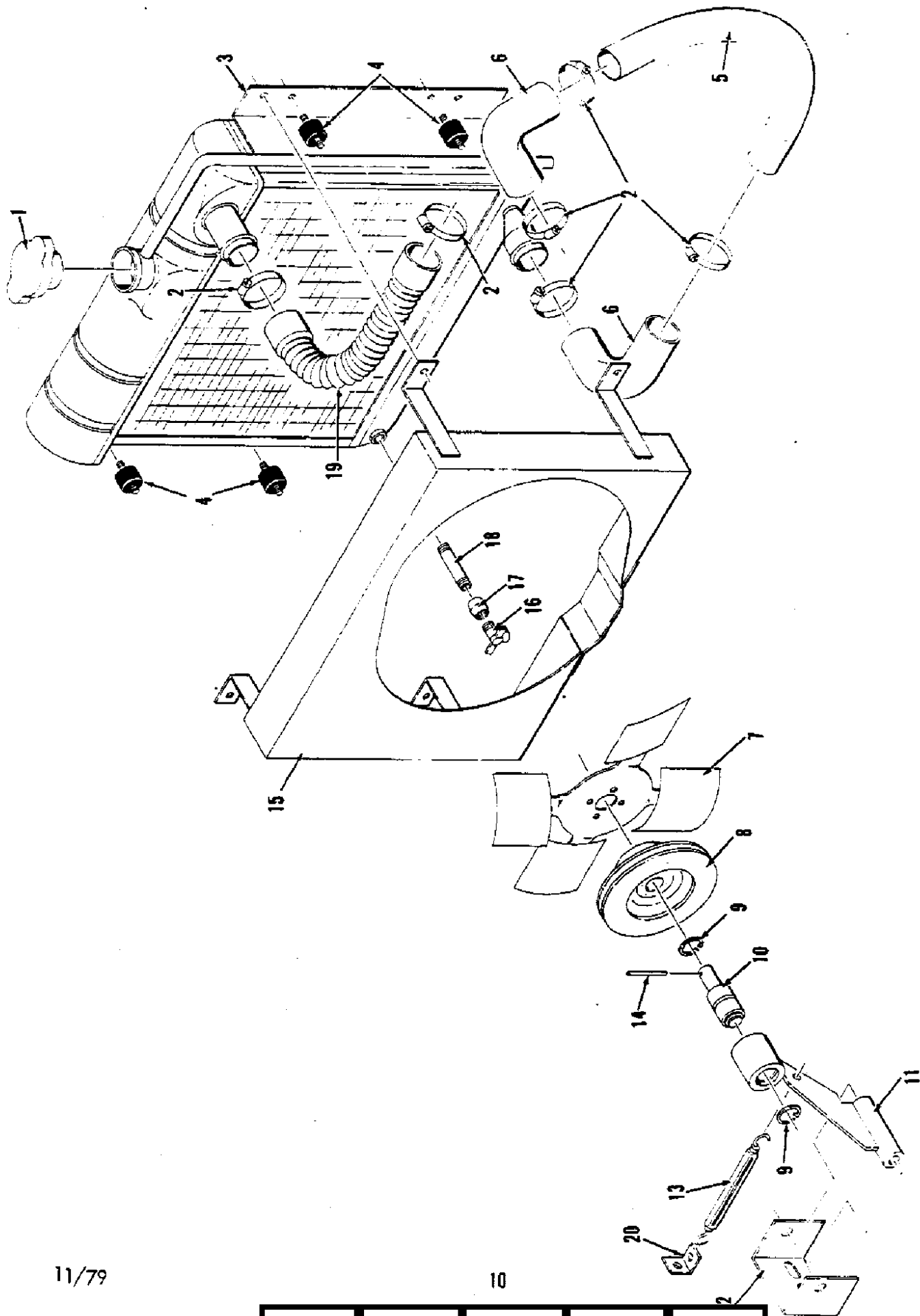
Fig. 5 - COOLING SYSTEM
