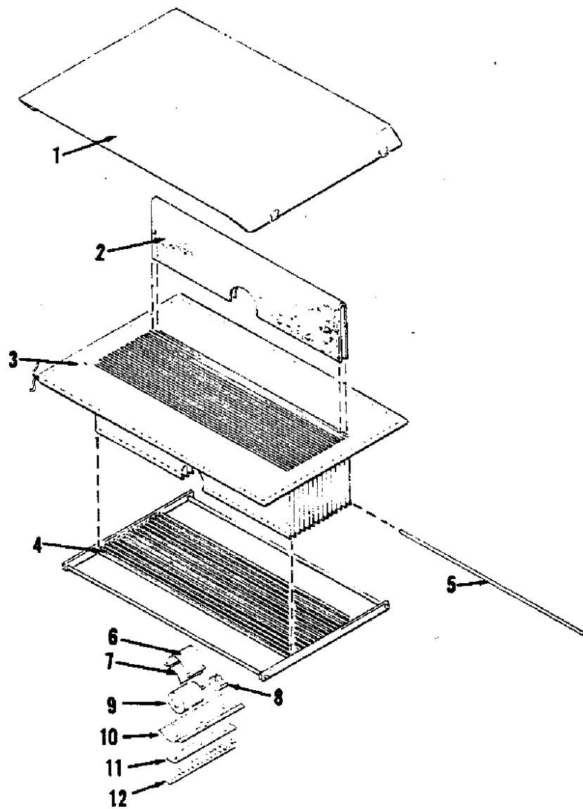
FIG. 6 - DUST FILTER &amp; SHAKER MOTOR
