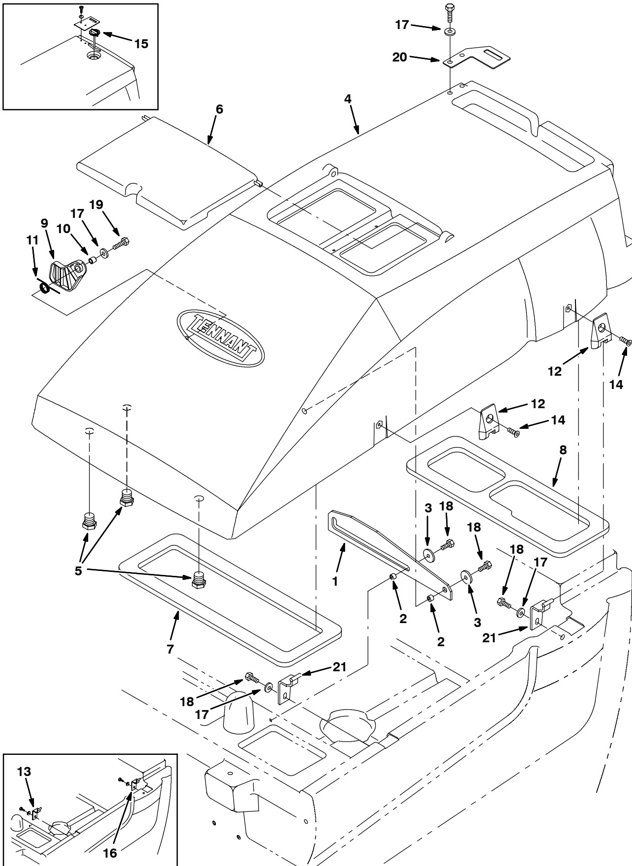
Fig. 11 - Solution Tank Group
