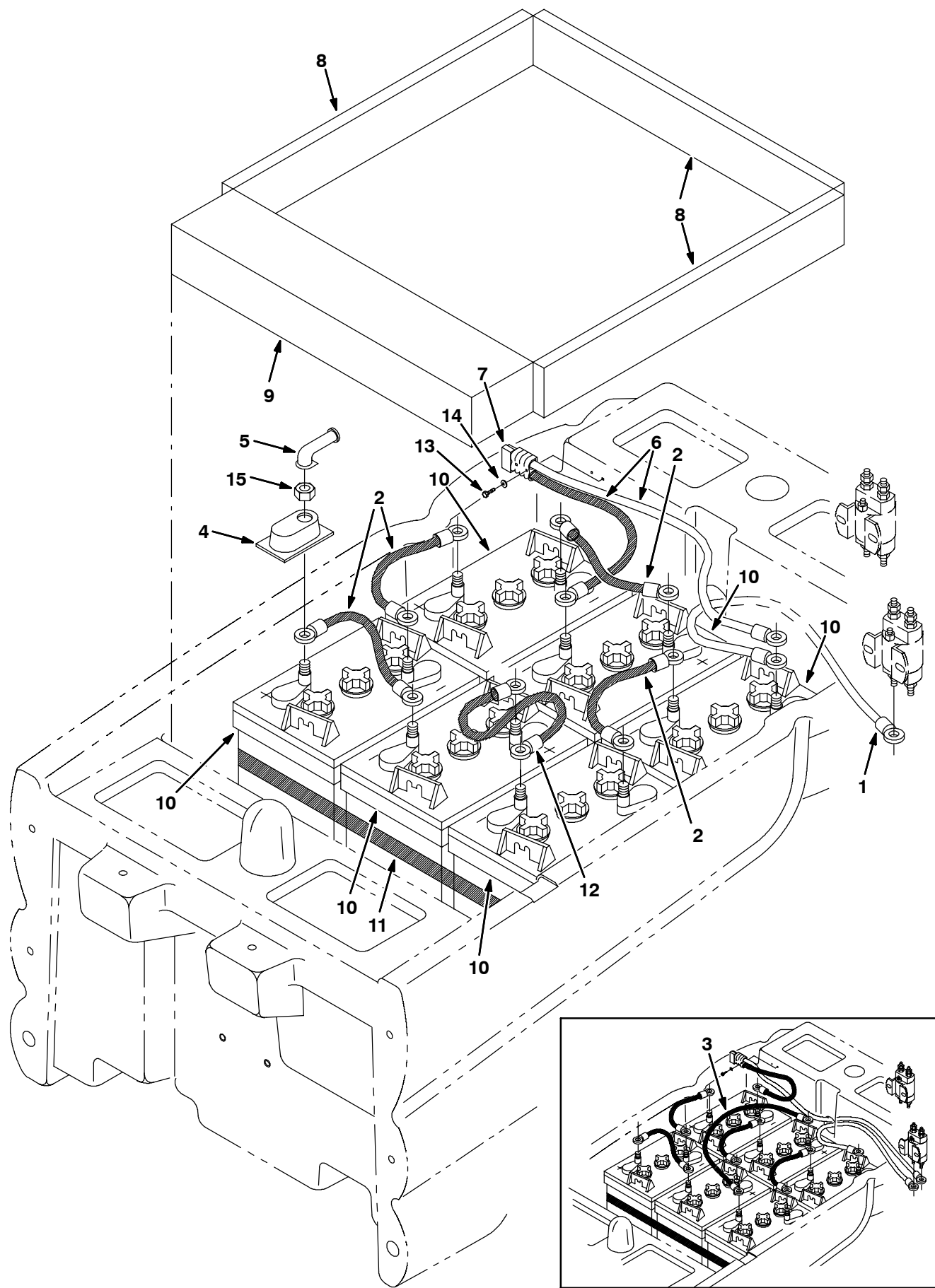
Fig. 14 - Battery Group
