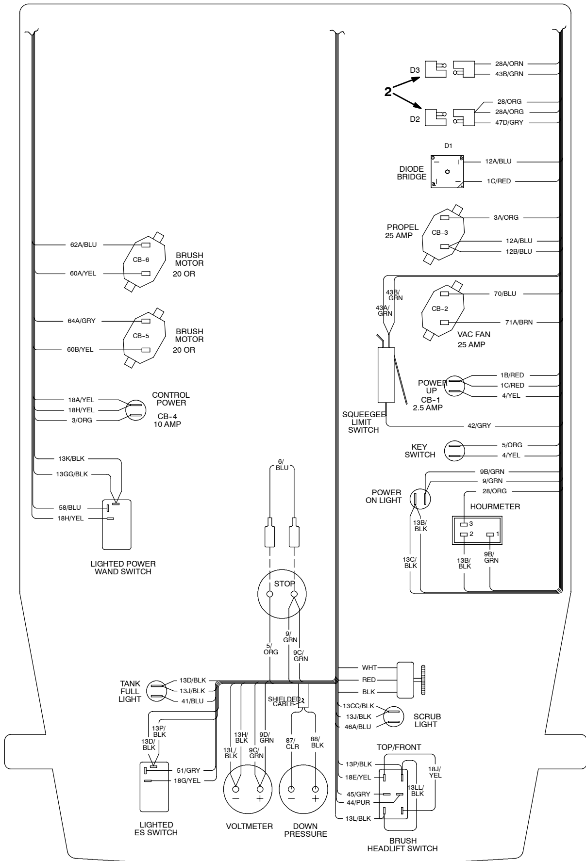
Fig. 23 - Electrical Wire Harness Group
