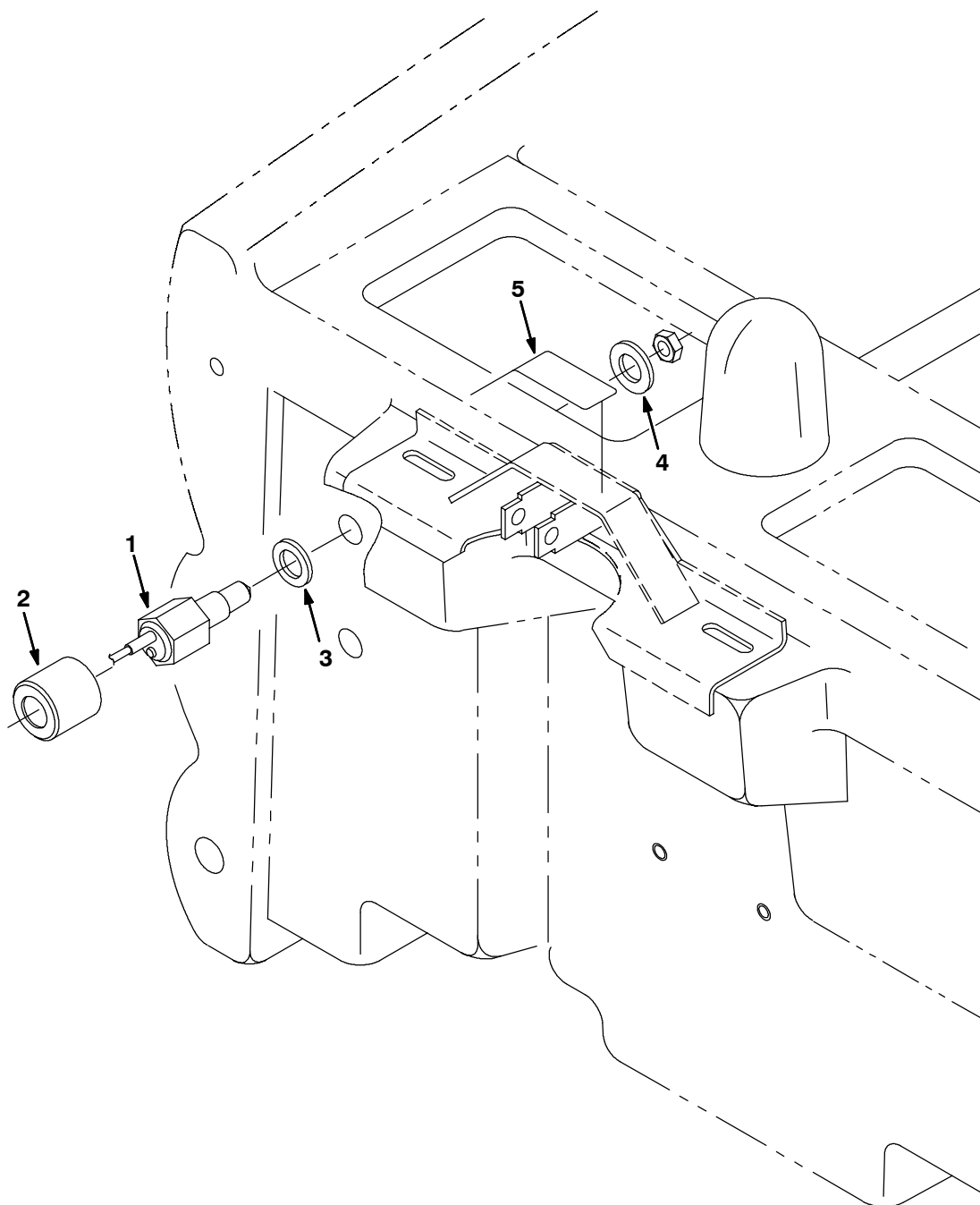
Fig. 17 - Sensor Kit, Optical (000000-xxxxxx)
