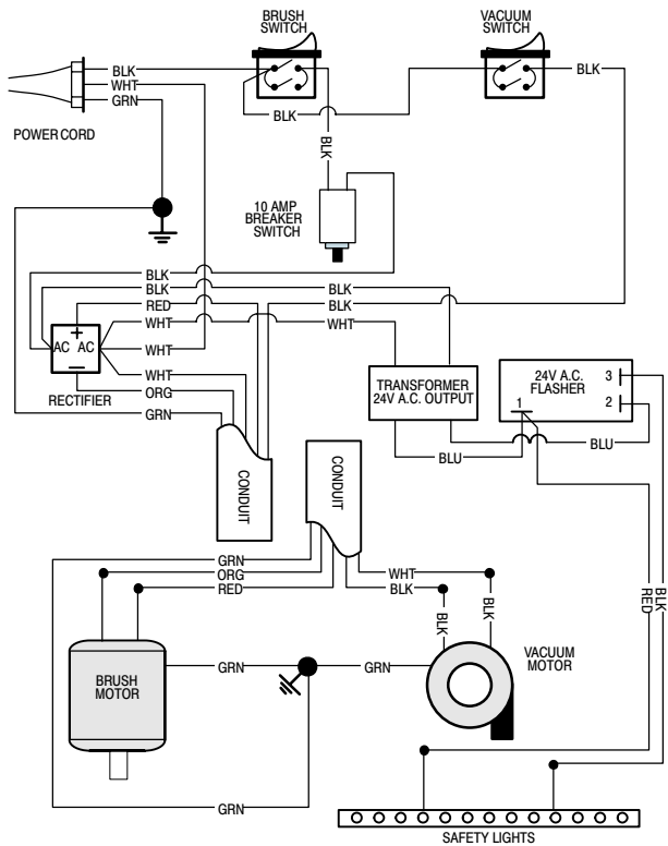
120V WIRE DIAGRAM
