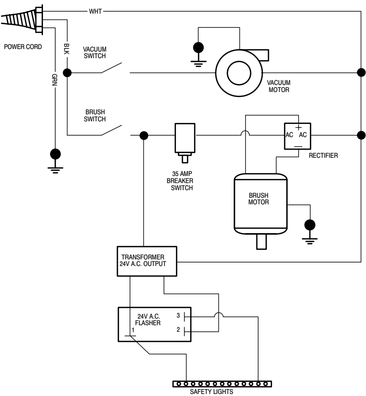
120V LADDER DIAGRAM
