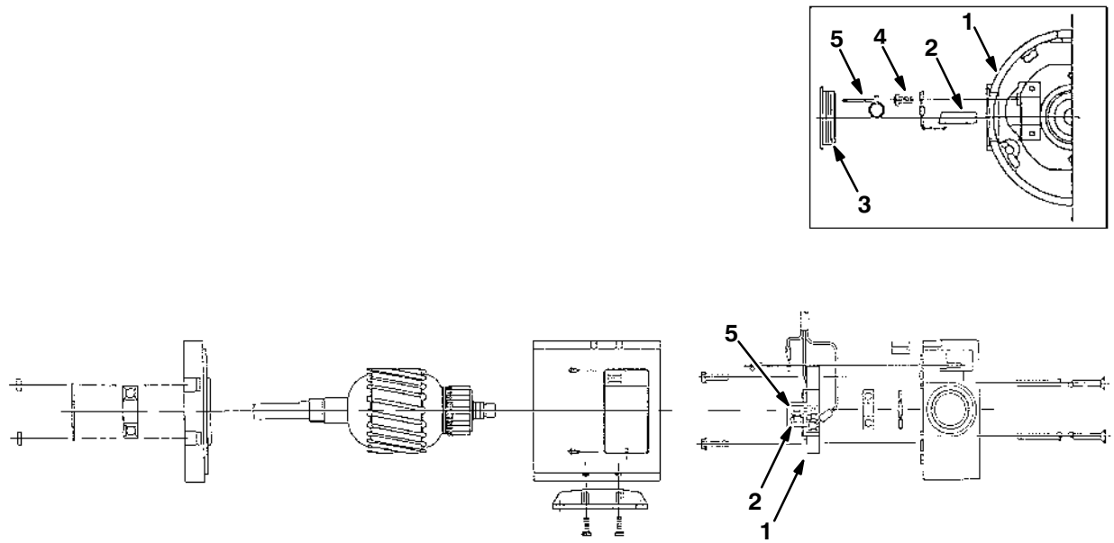
Fig. 3 – Brush Motor
