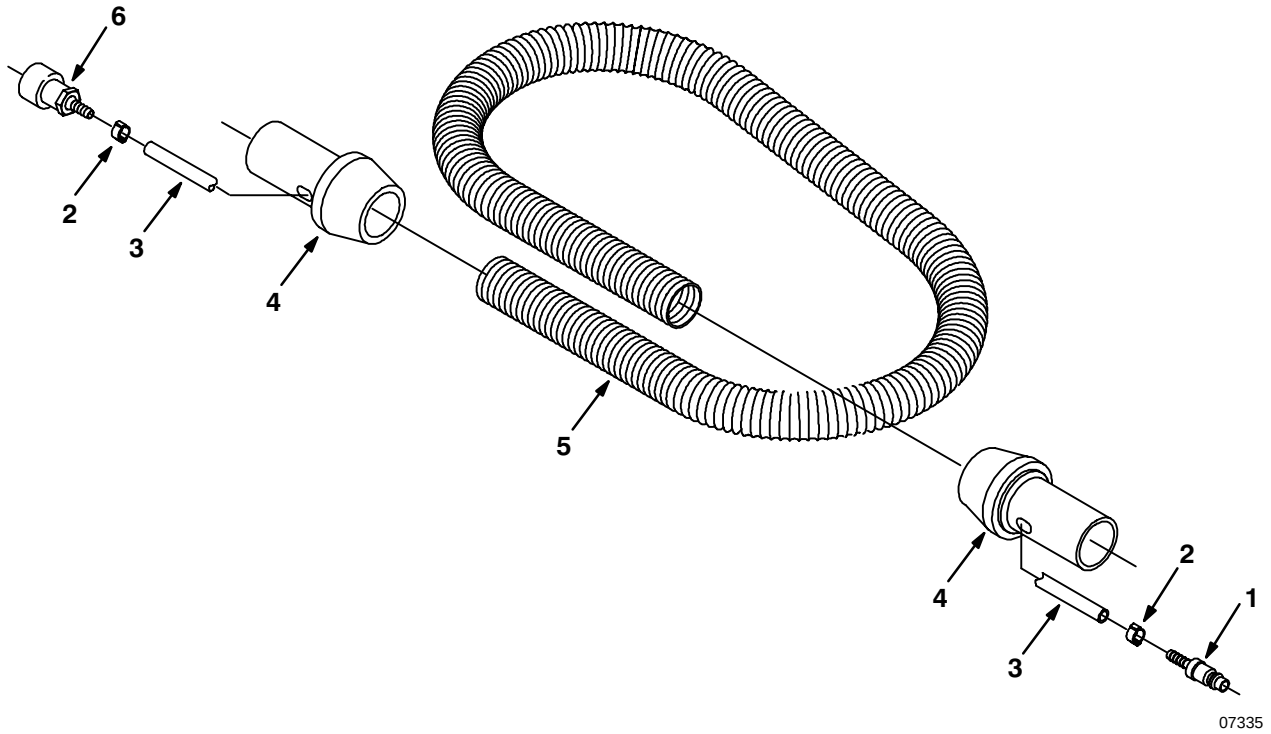
Fig. 2 – Hose Assembly
