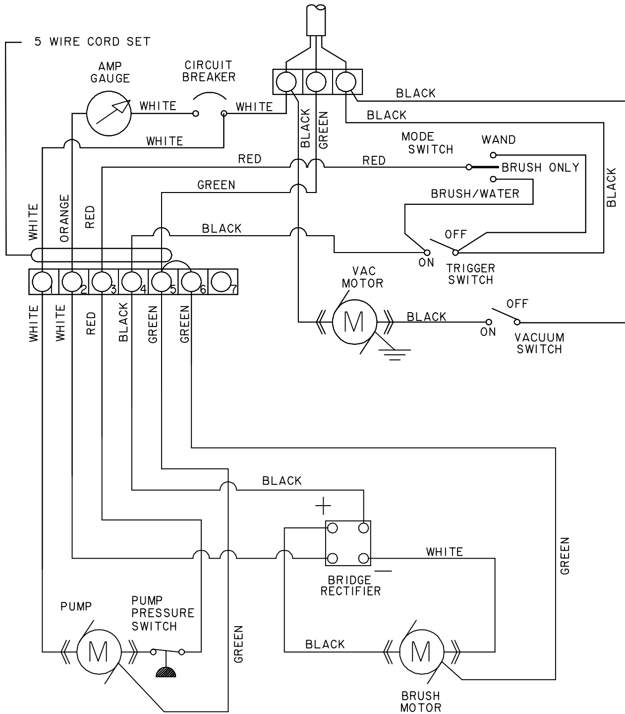
Fig. 6 – Electrical Schematic
