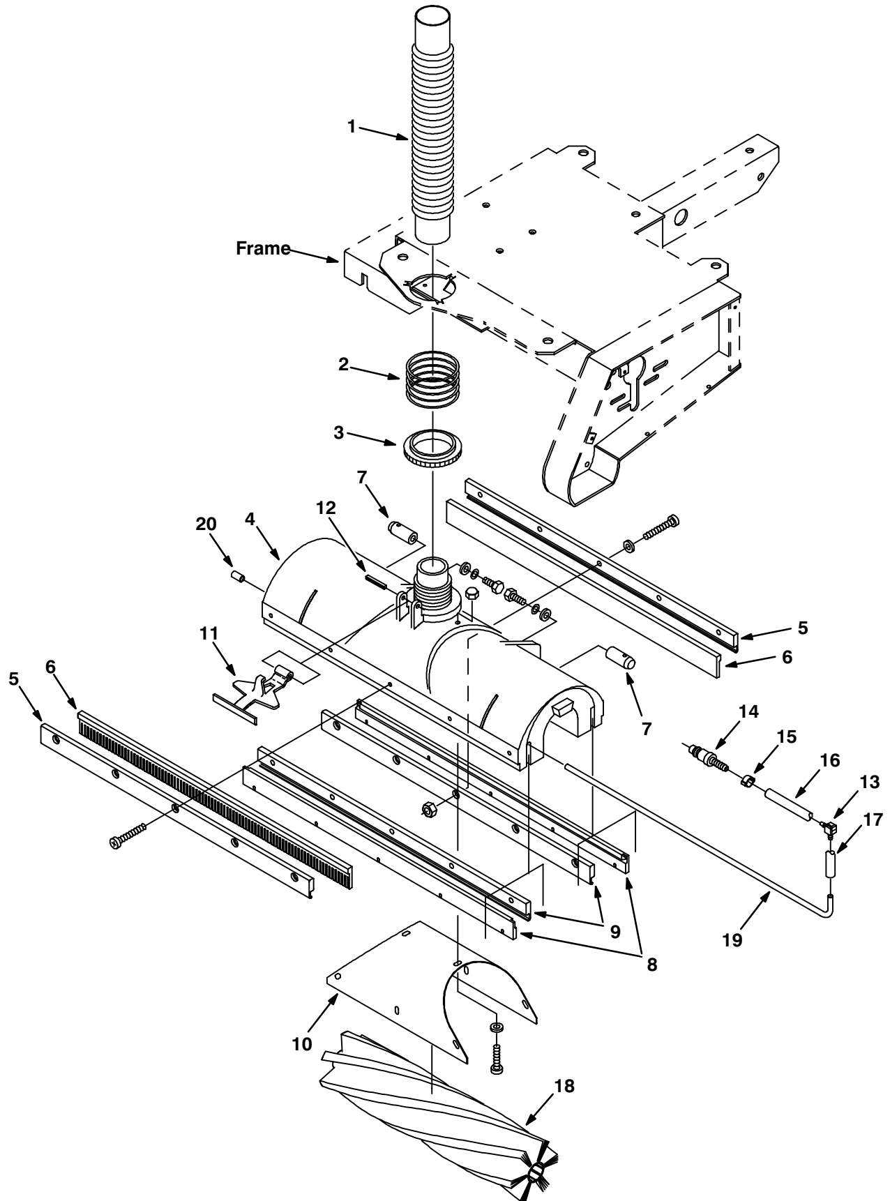
Fig. 4 – Squeegee Head Group
