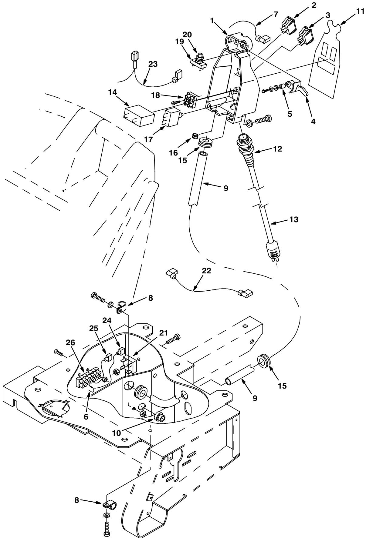
Fig. 5 - Electrical Panel
