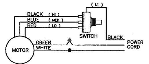
WIRING DIAGRAM
