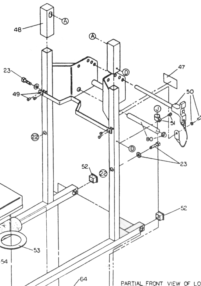
PARTIAL FRONT VIEW OF LOWER FRAME
