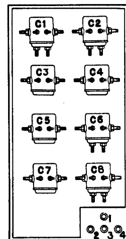
CONTACTOR LOCATION
