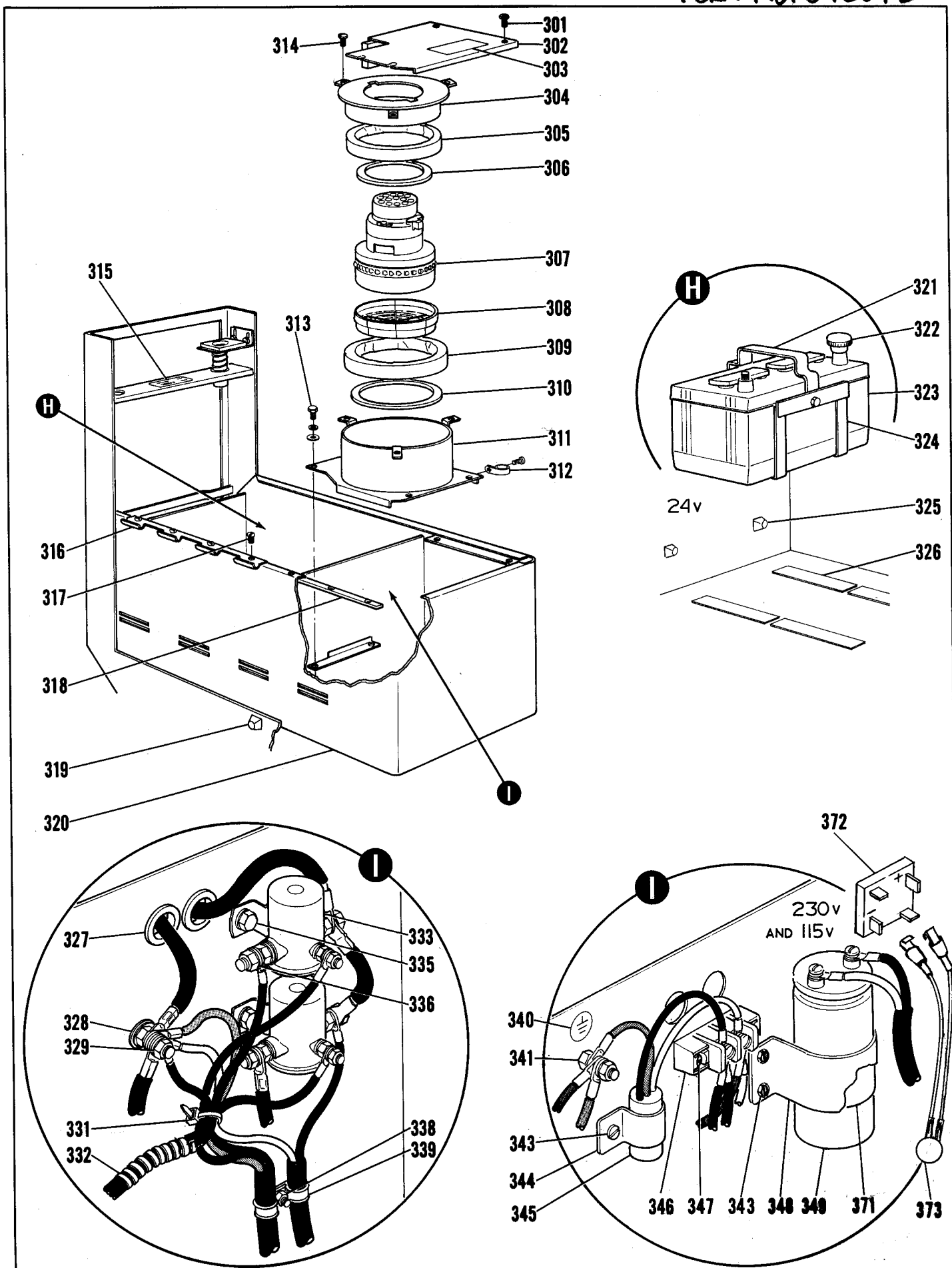
HOUSING ASSEMBLY
