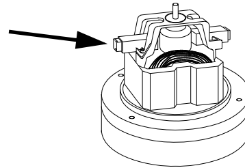
Carbon Brushes
