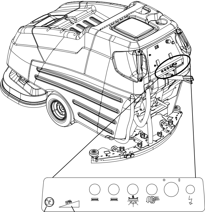
CIRCUIT BREAKER DECAL 86243530 PRV NO. 500565
