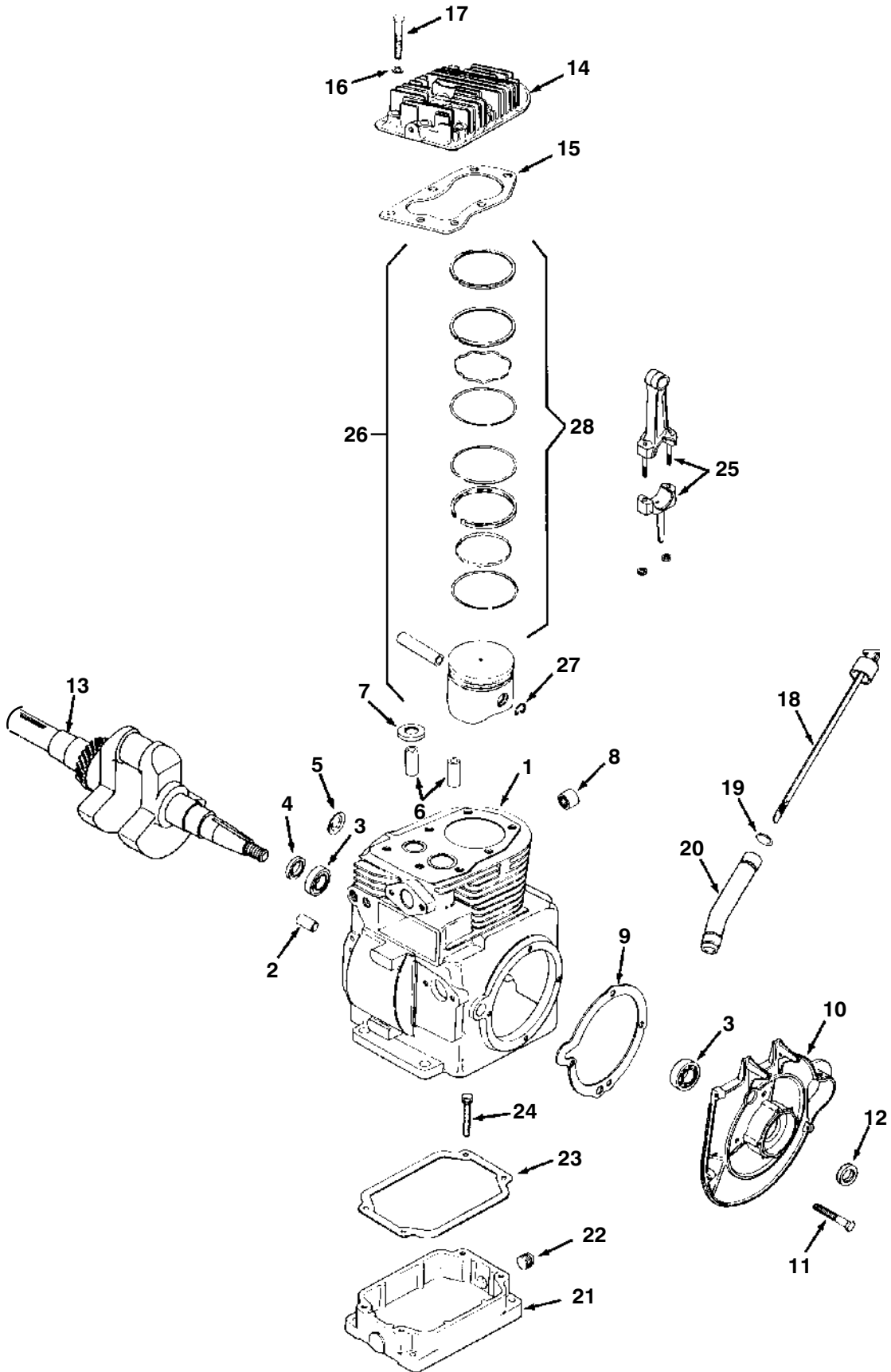
Fig. 1 – Crankcase Group
