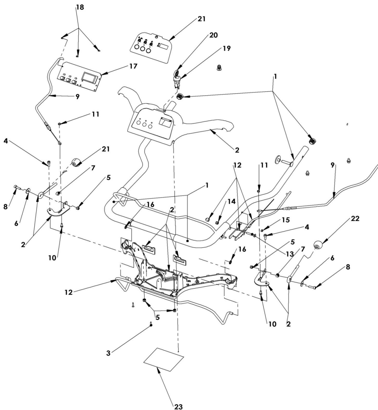
Fig. 7 – Handle Assy
