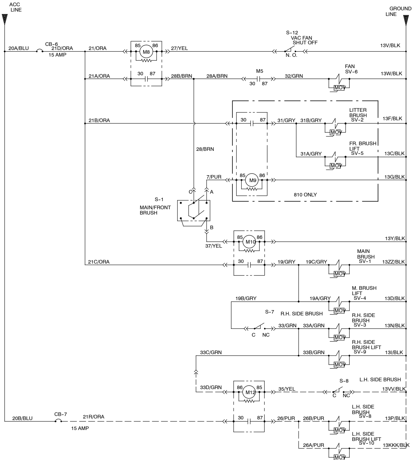
Fig. 59 - Electrical Schematic (004000- 004302)
