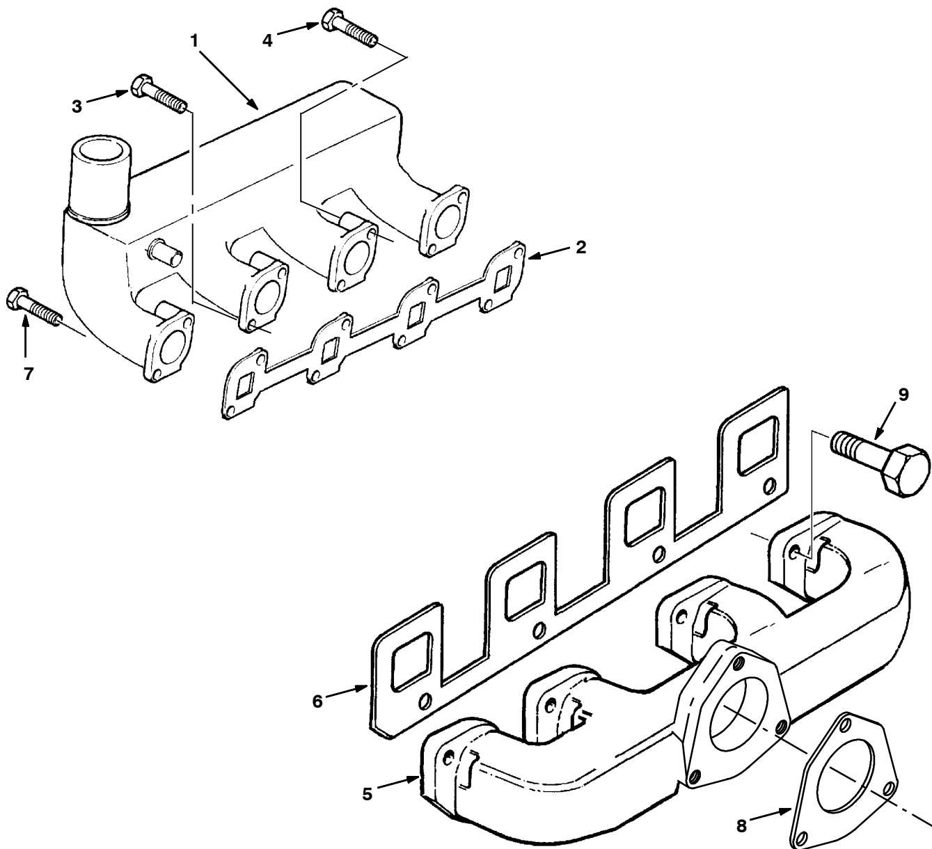
Fig. 16 - Manifold Group
