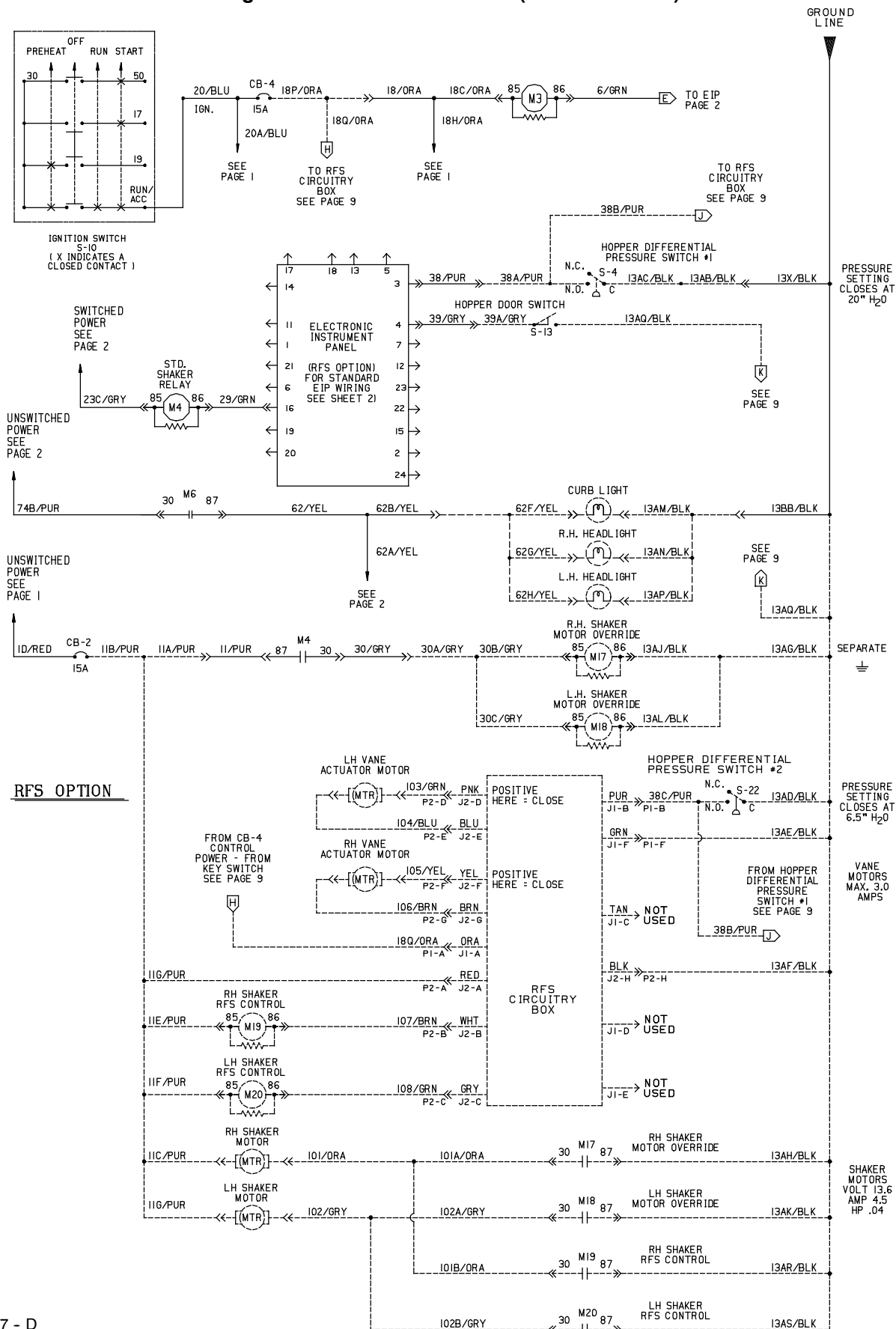
Fig. 60 - Electrical Schematic (004303-006008)
