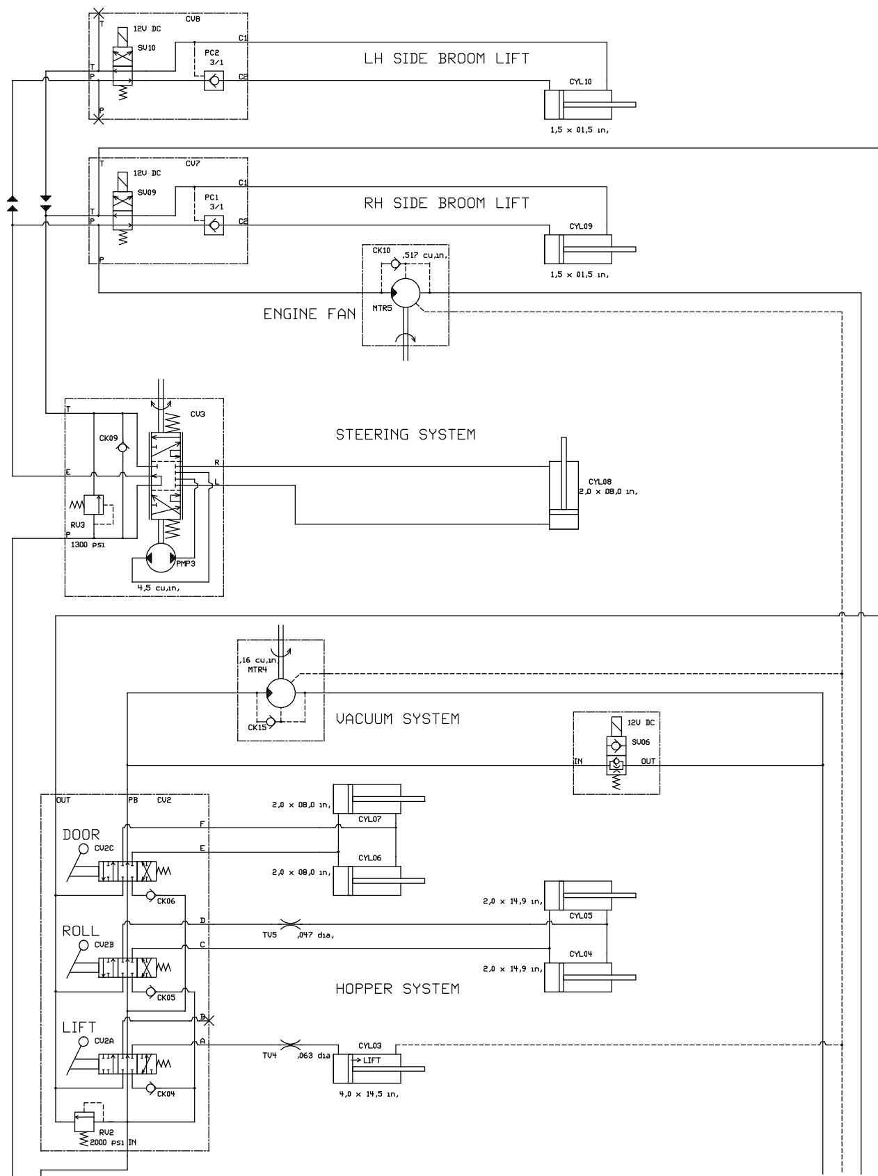
Fig. 43 - Hydraulic Schematic
