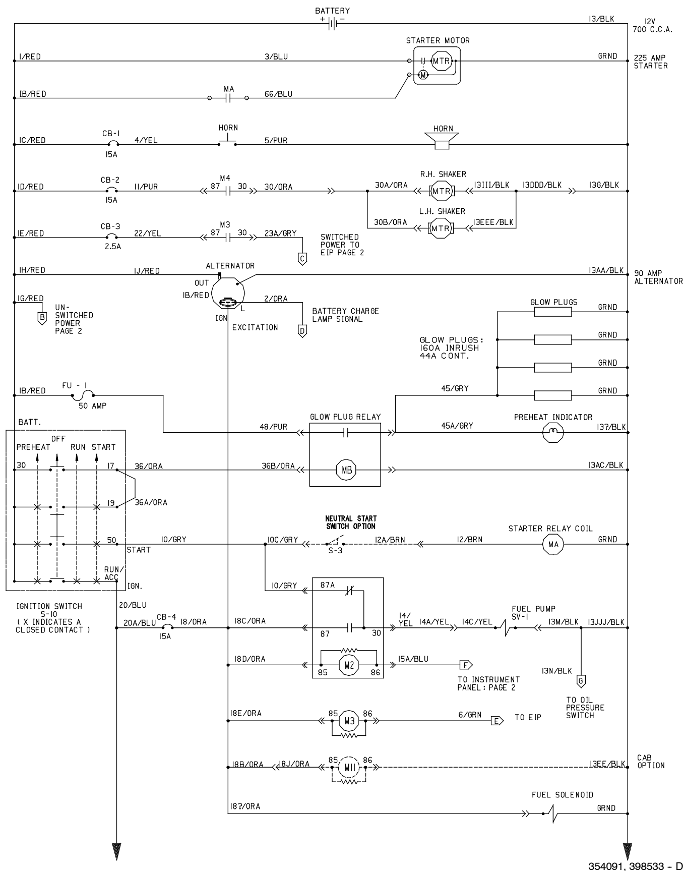
Fig. 61 - Electrical Schematic (006009- )
