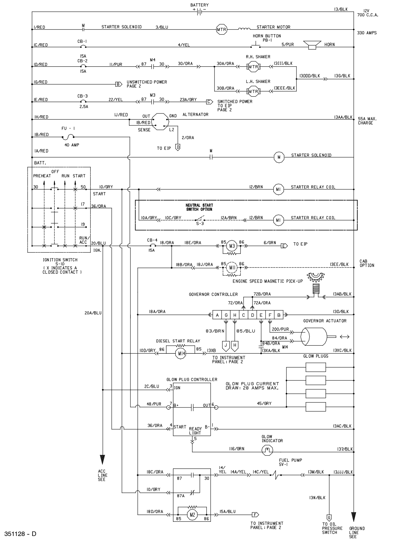
Fig. 60 - Electrical Schematic (004303-006008)
