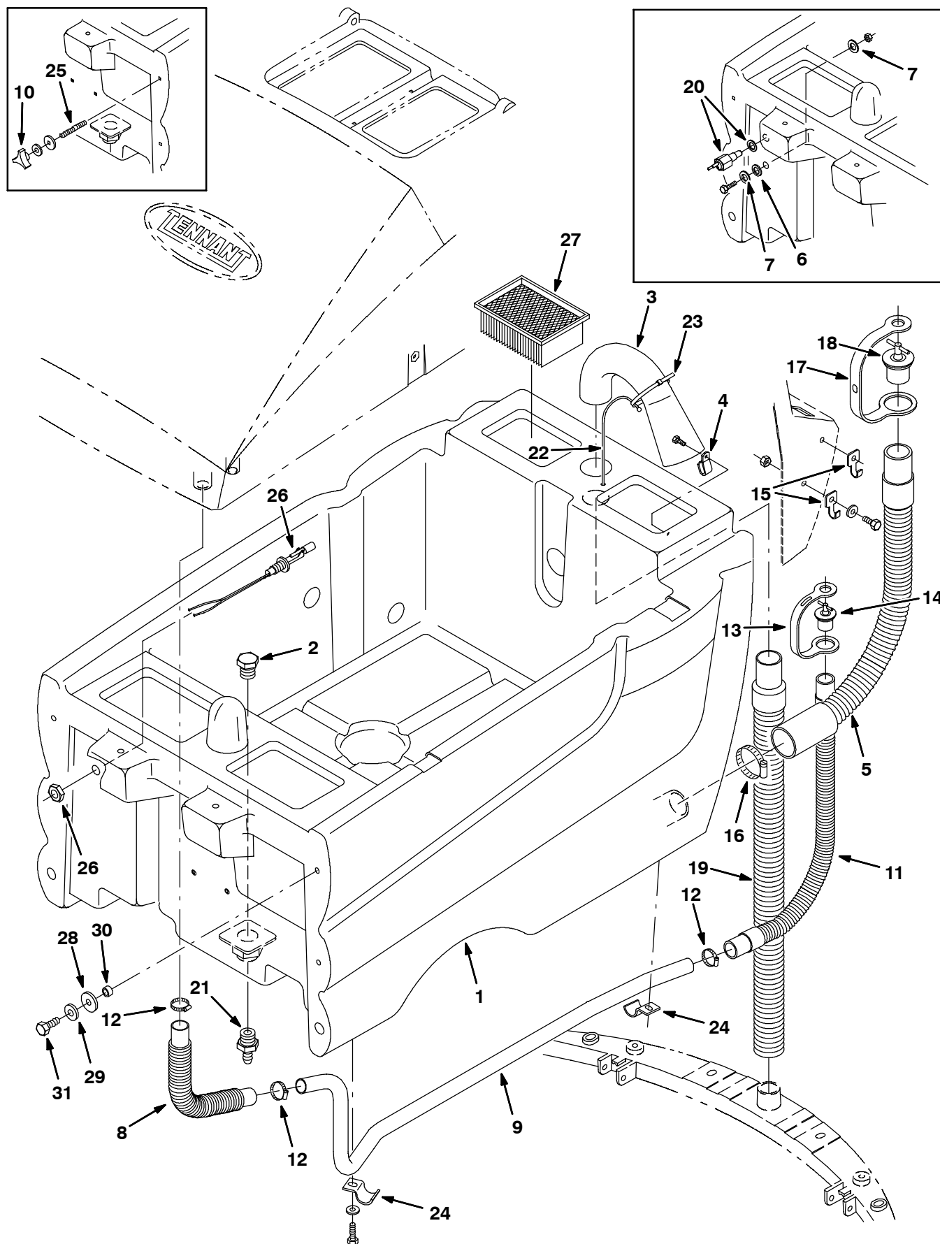
Fig. 19 - Recovery Tank Group (57150 0001-xxxx) - Schmutzwasser Tank Gruppe (57150 0001-xxxx) - Groupe Reservoir de Recouvrer (57150 0001-xxxx)
