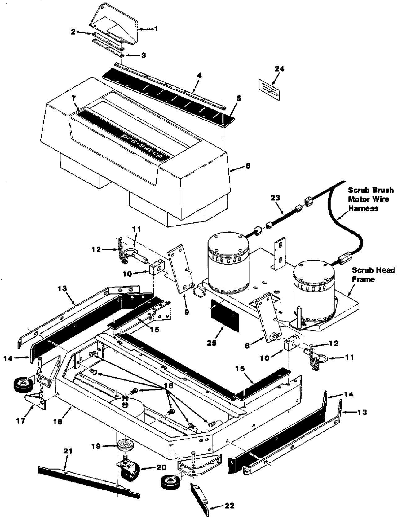
Fig. 15 - Pre-Sweep Group
