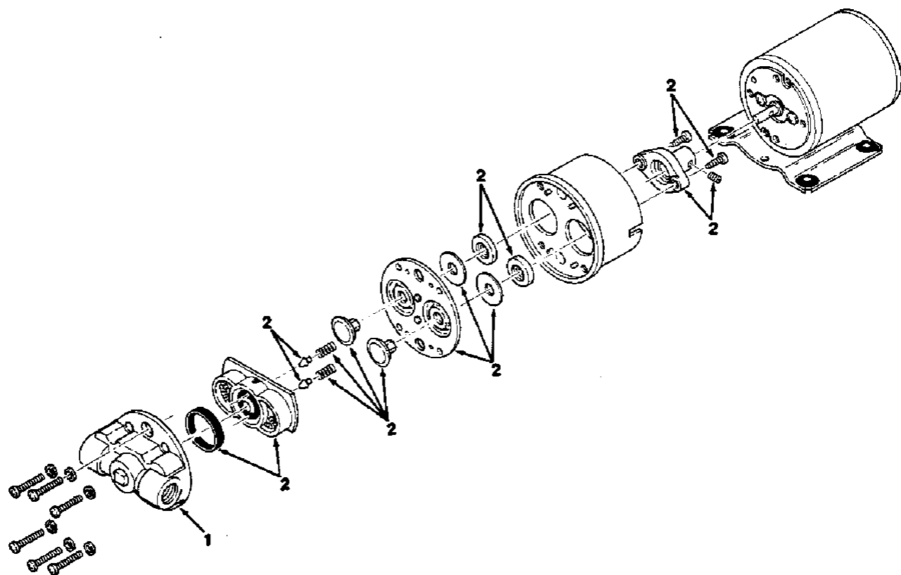
Fig. 6 – Water Pump Breakdown
