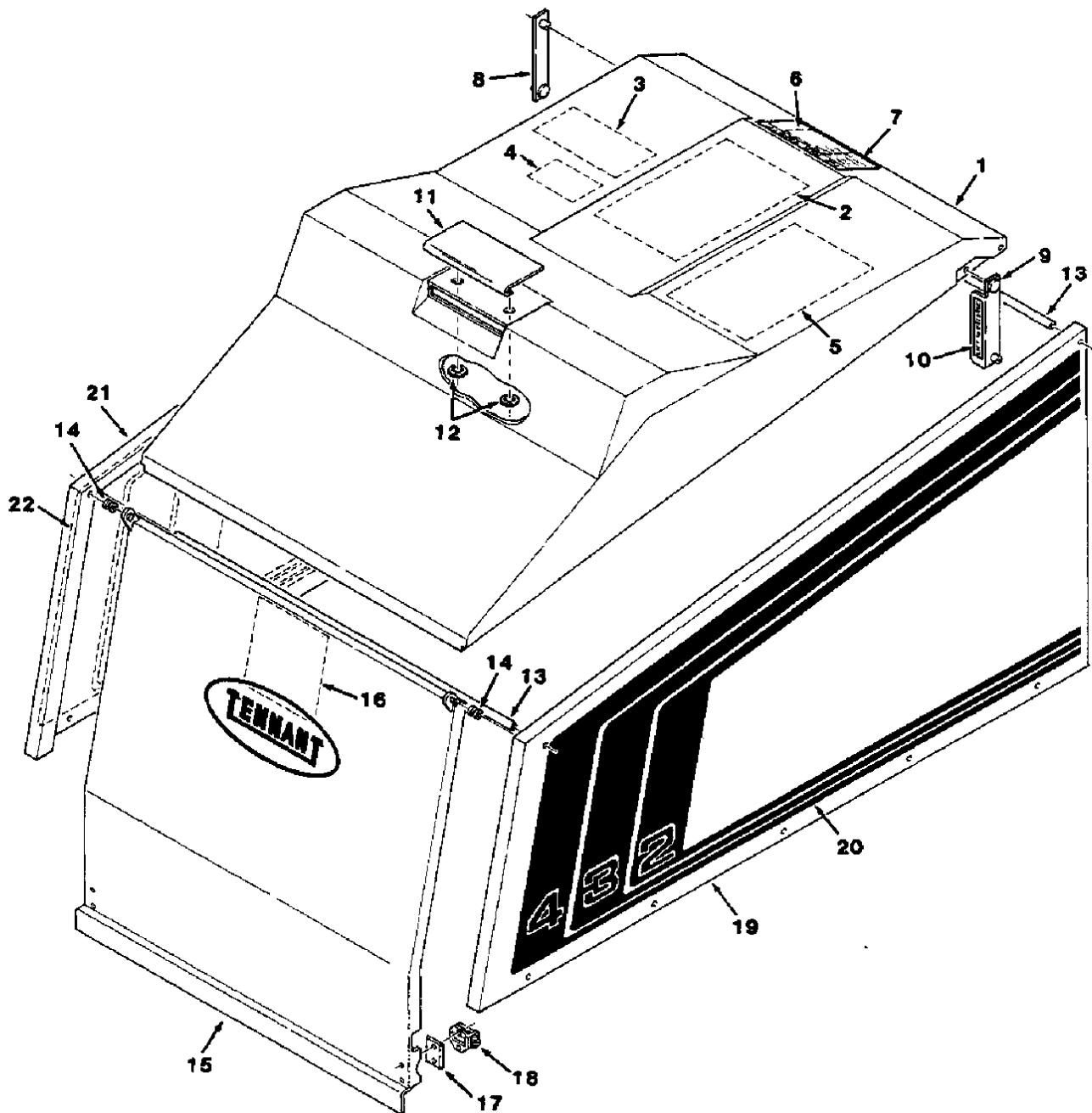
Fig. 5 - Hood and Covers Group
