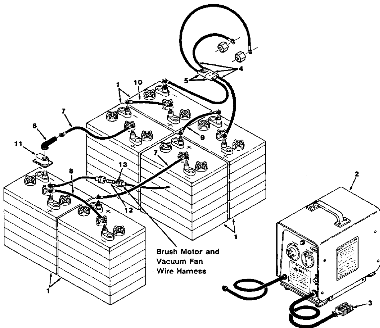
Fig. 16 - Battery Group
