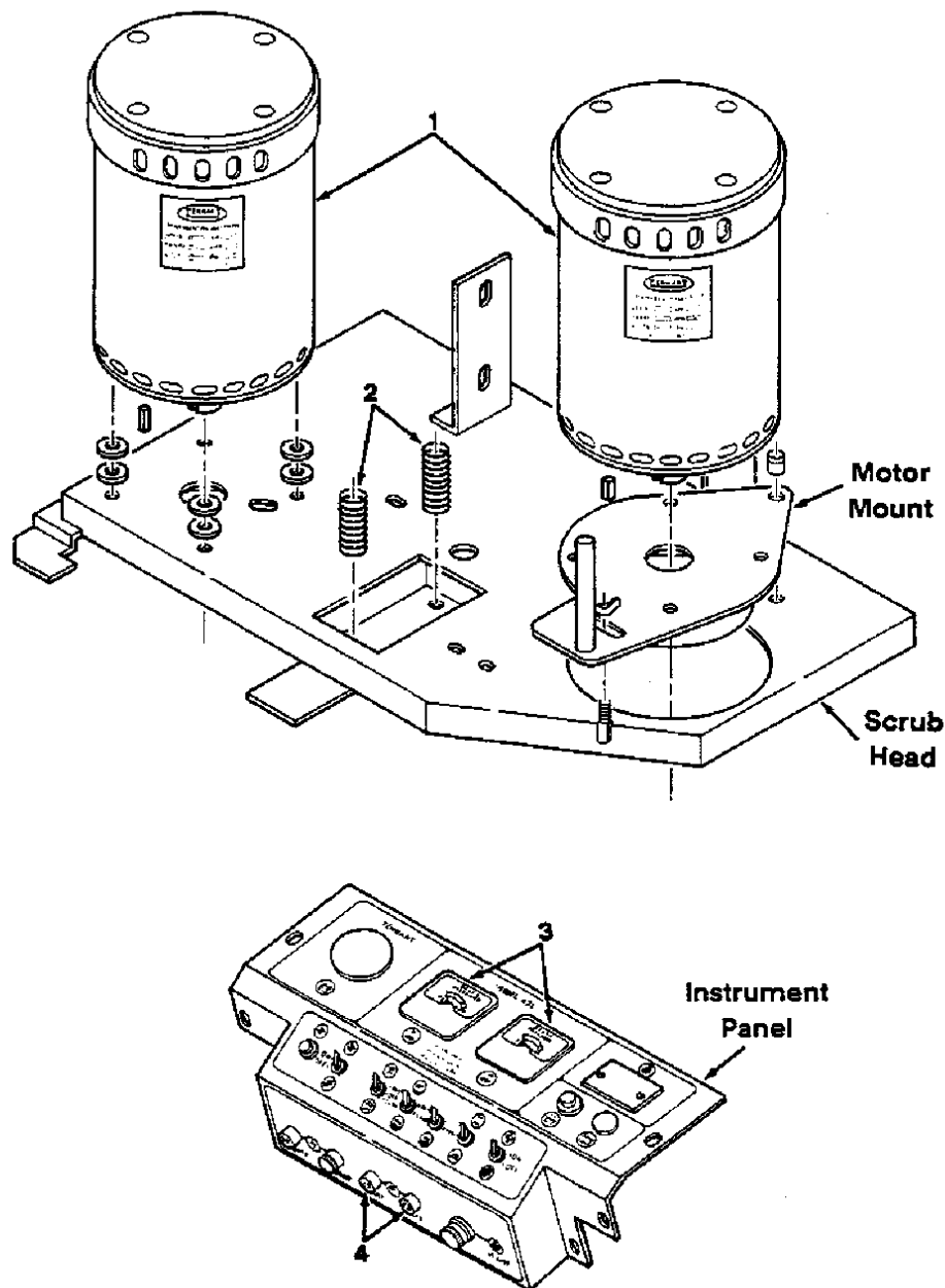
Fig. 5 - Motor Kit, Heavy Duty
