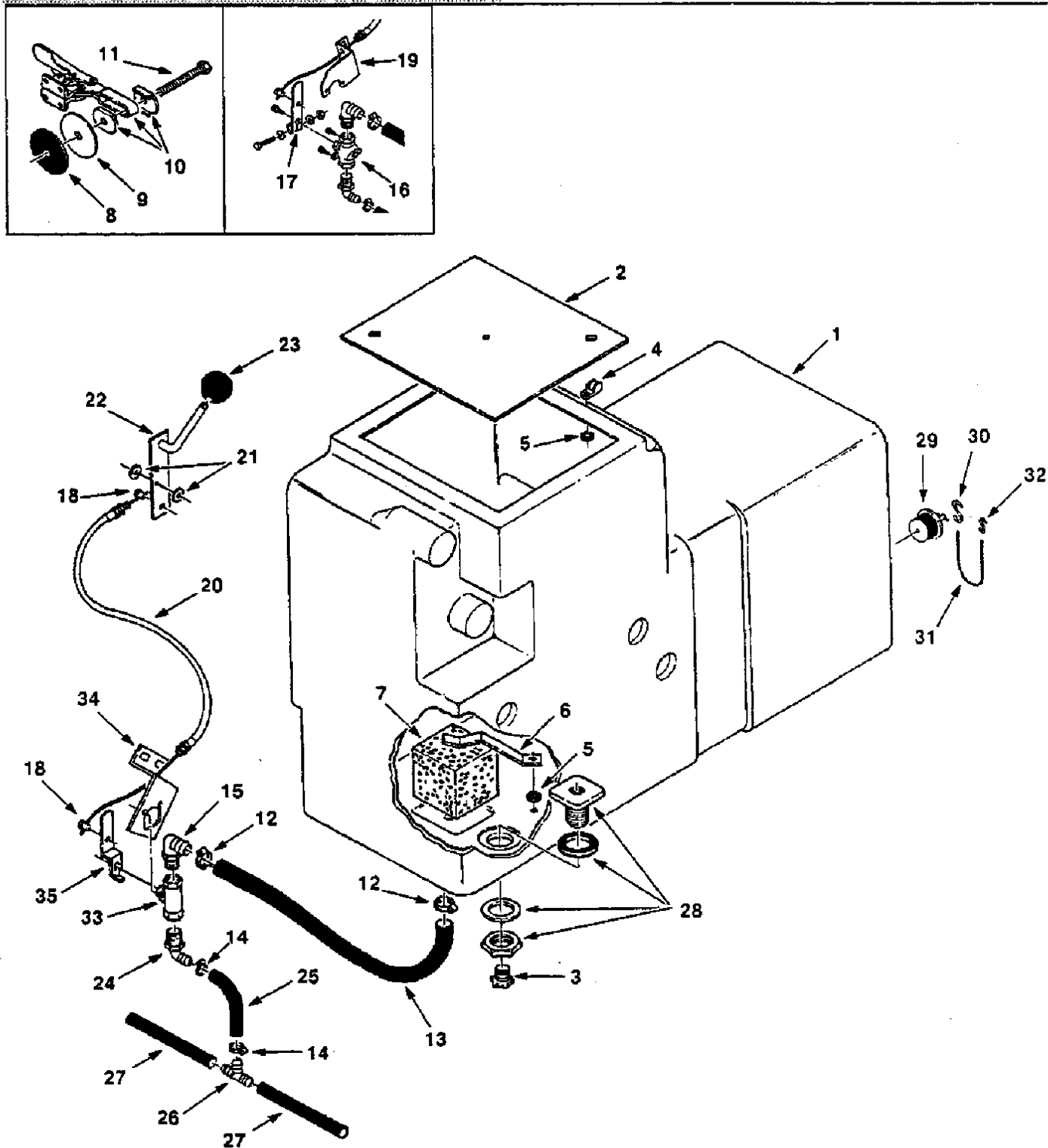
Fig. 11 - Solution Tank and Control Group
