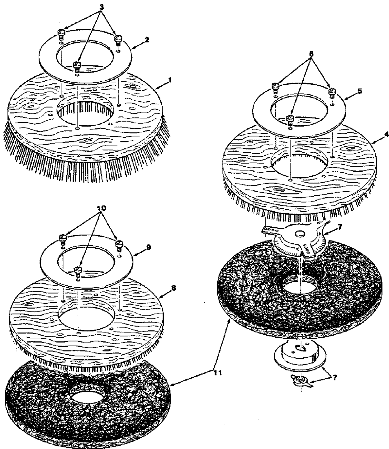
Fig. 1 ~ Replacement Brushes
