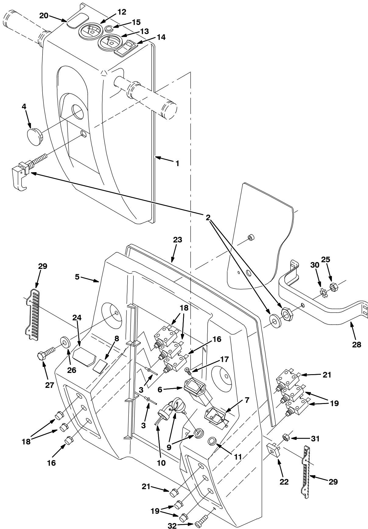
Fig. 27 - Operator Console Group
