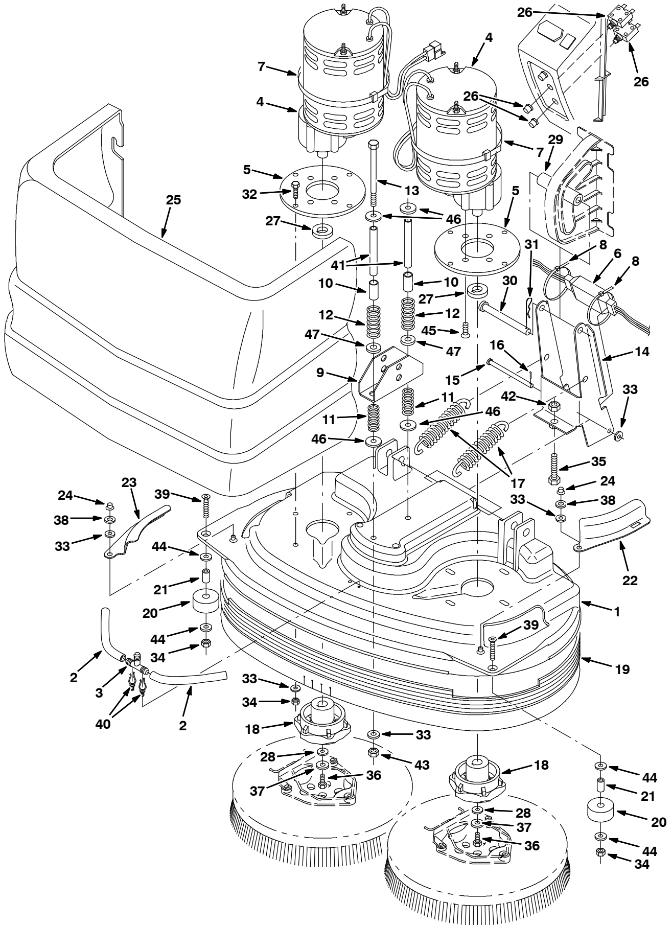
Fig. 14 - Scrub Head Kit, Model 800D Heavy Duty, 800 mm (32 in) (S/N 10000000- 10547657)
