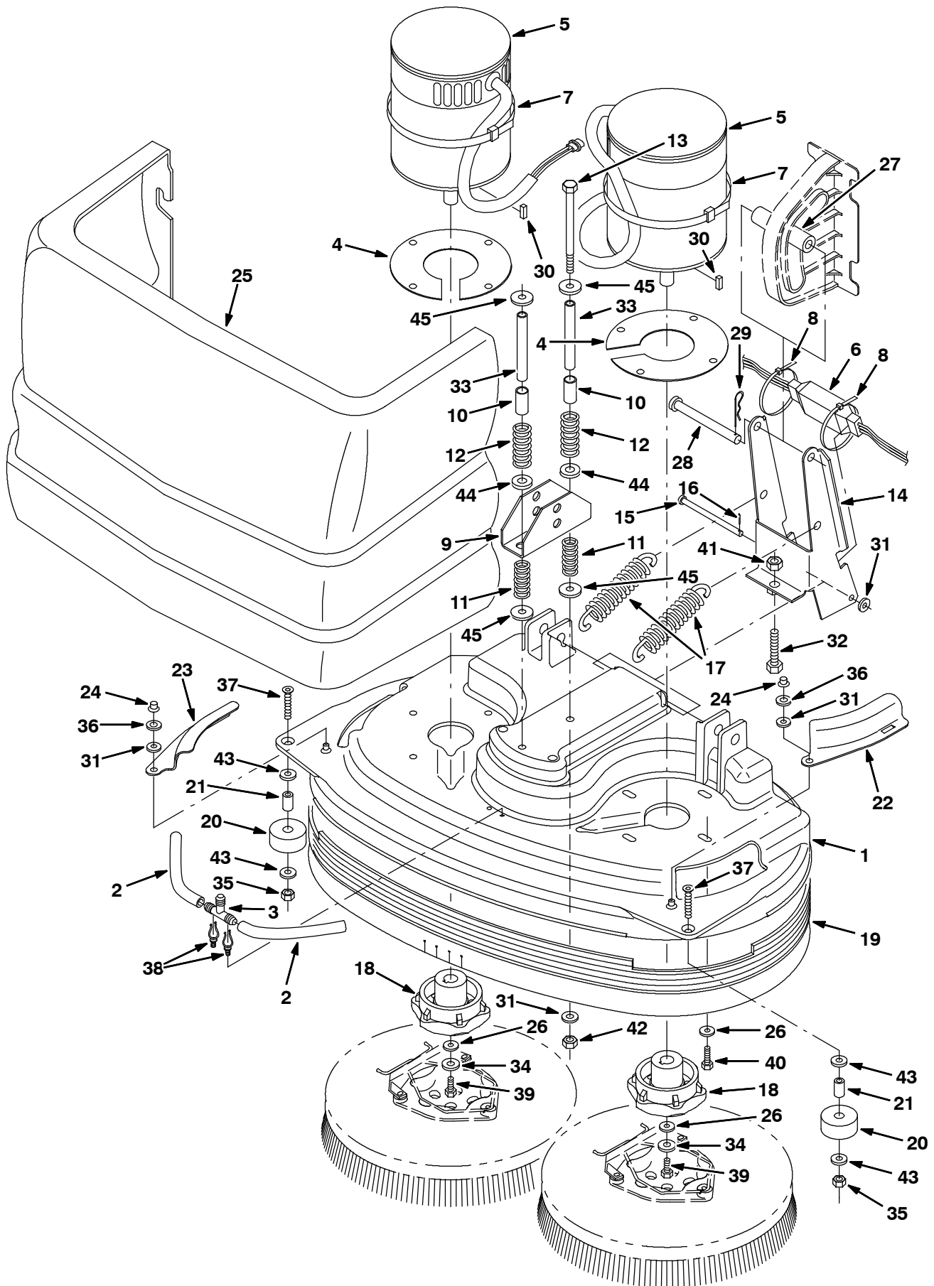
Fig. 10 - Scrub Head Kit, Model 800D, 800 mm (32 in) (S/N 10000000- 10570246)
