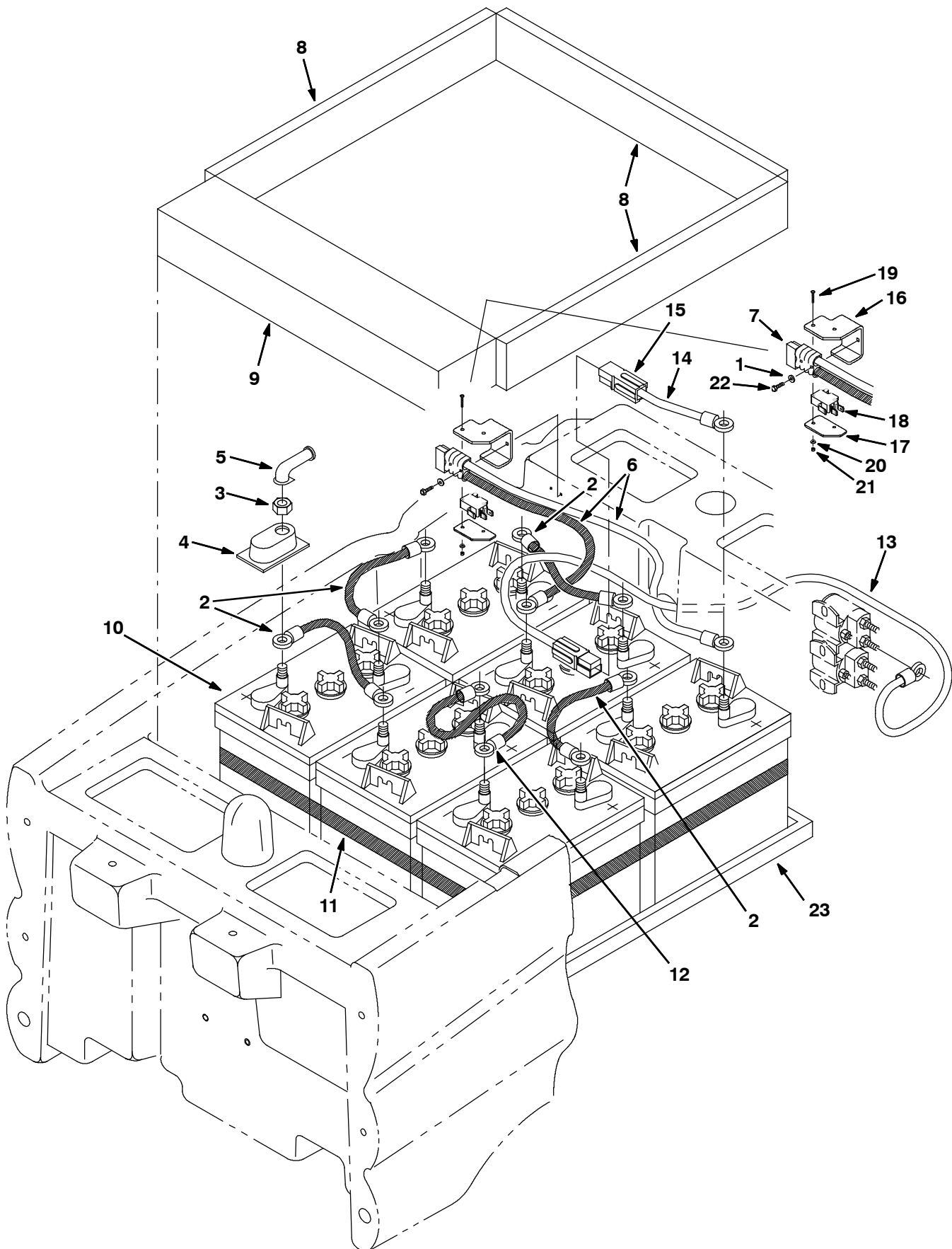
Fig. 25 - Battery Group
