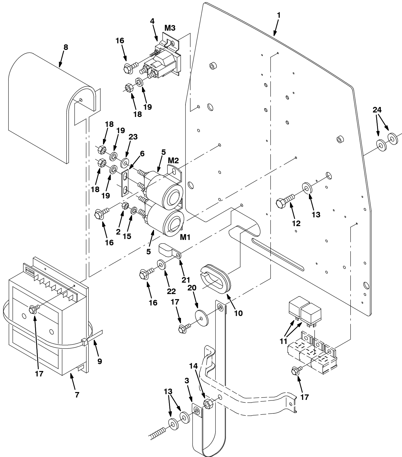
Fig. 28 - Electrical Panel Group
