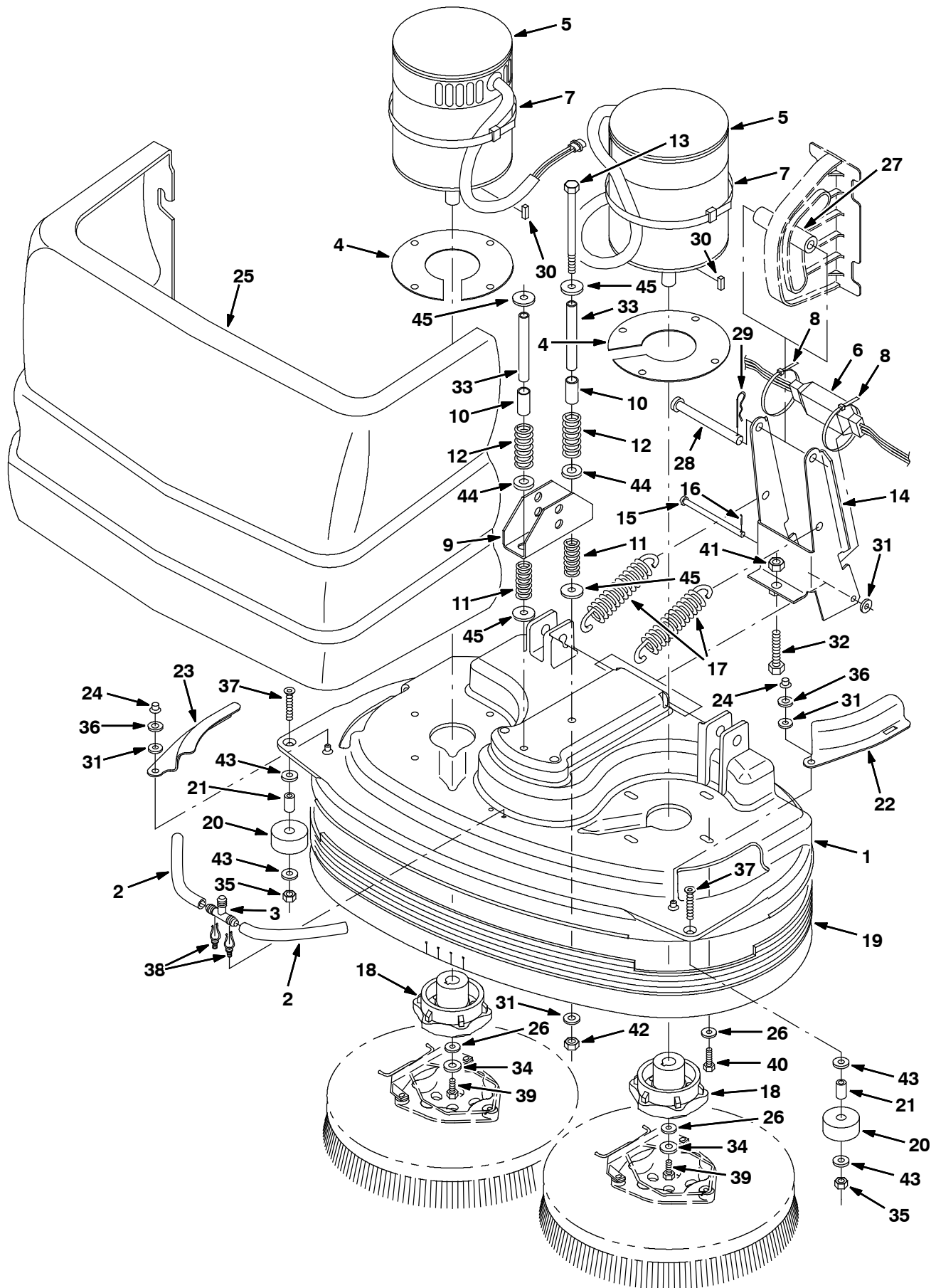
Fig. 8 - Scrub Head Kit, Model 700D, 700 mm (28 in) (S/N 10000000- 10570246)
