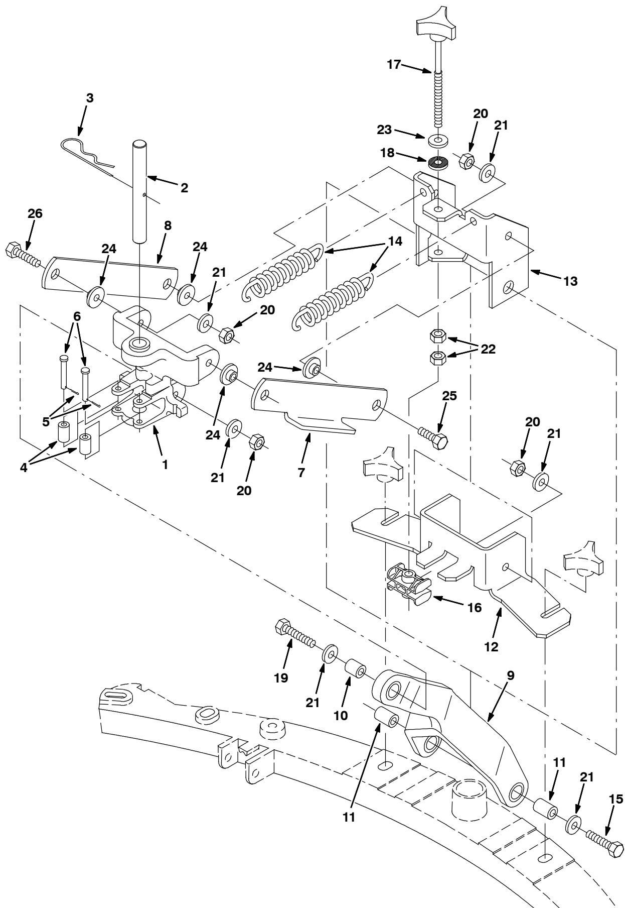
Fig. 30 - Squeegee Linkage Group
