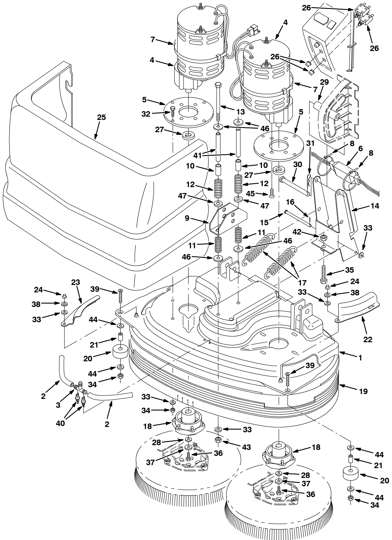
Fig. 12 - Scrub Head Kit, Model 900D, 900 mm (36 in) (S/N 10000000- 10547659)
