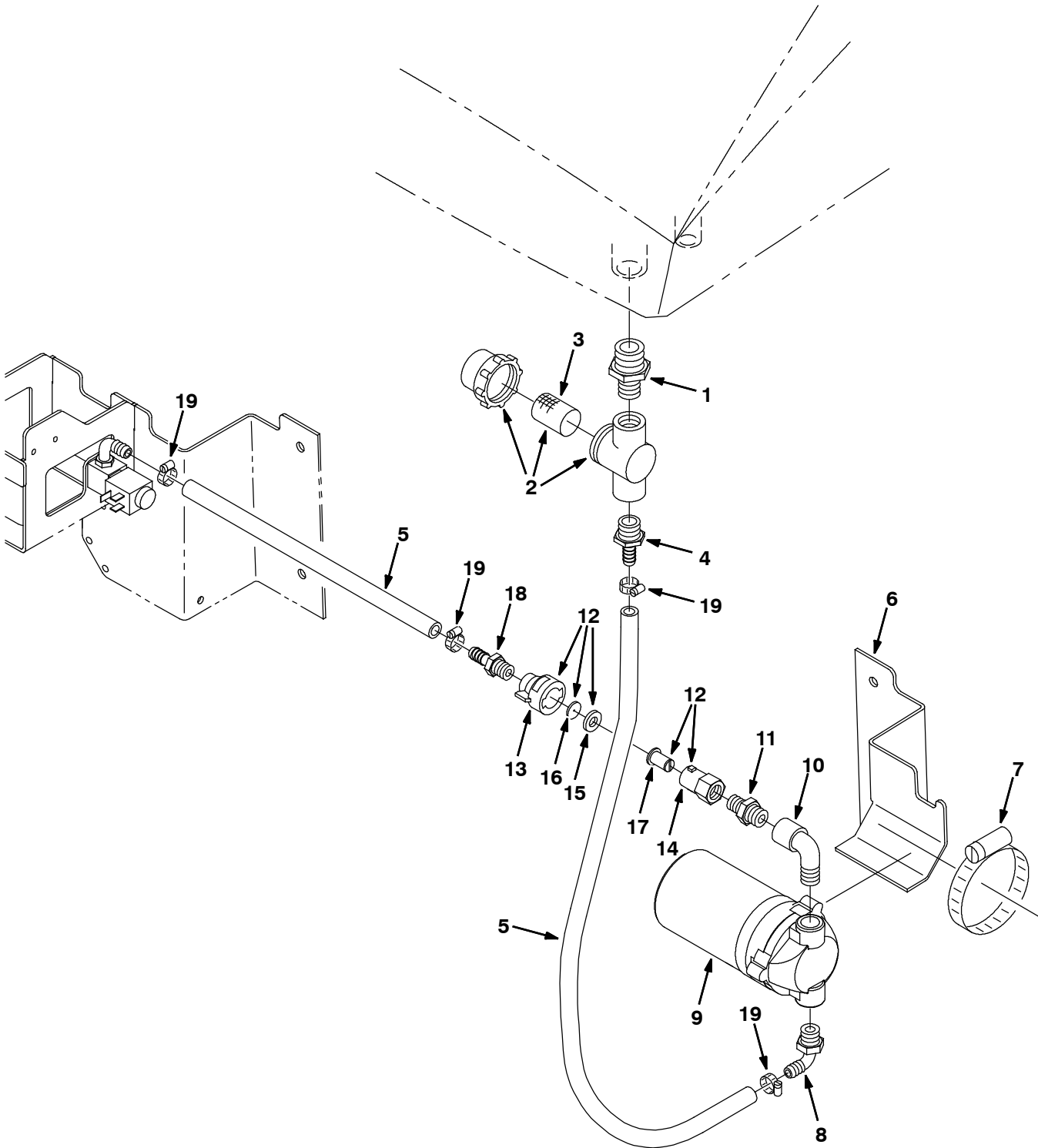
Fig. 11 - FaST Solution Pump Group (S/N 10000000 - 10361712)
