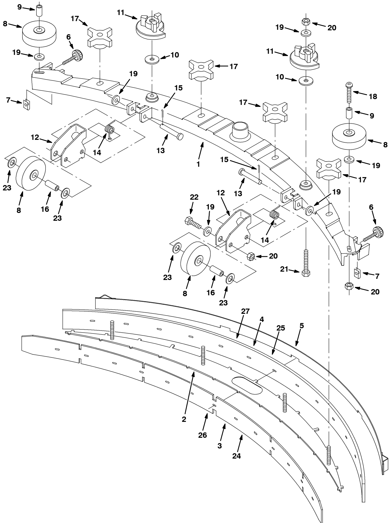
Fig. 34 - Squeegee Group, Model 900, 900 mm (36 in)
