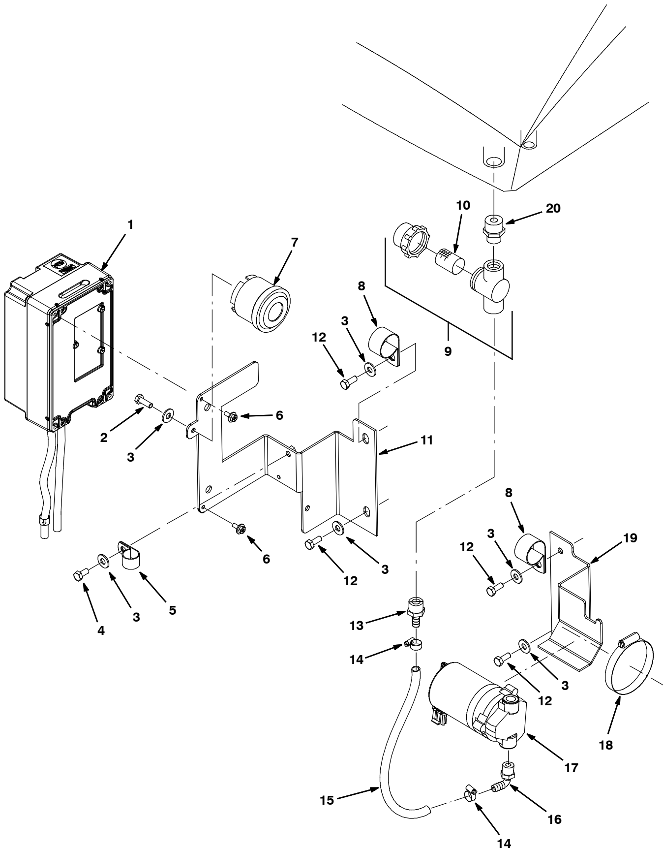
Fig. 18 - ec-H2O Solution Pump Group (S/N 10000000-10581869)
