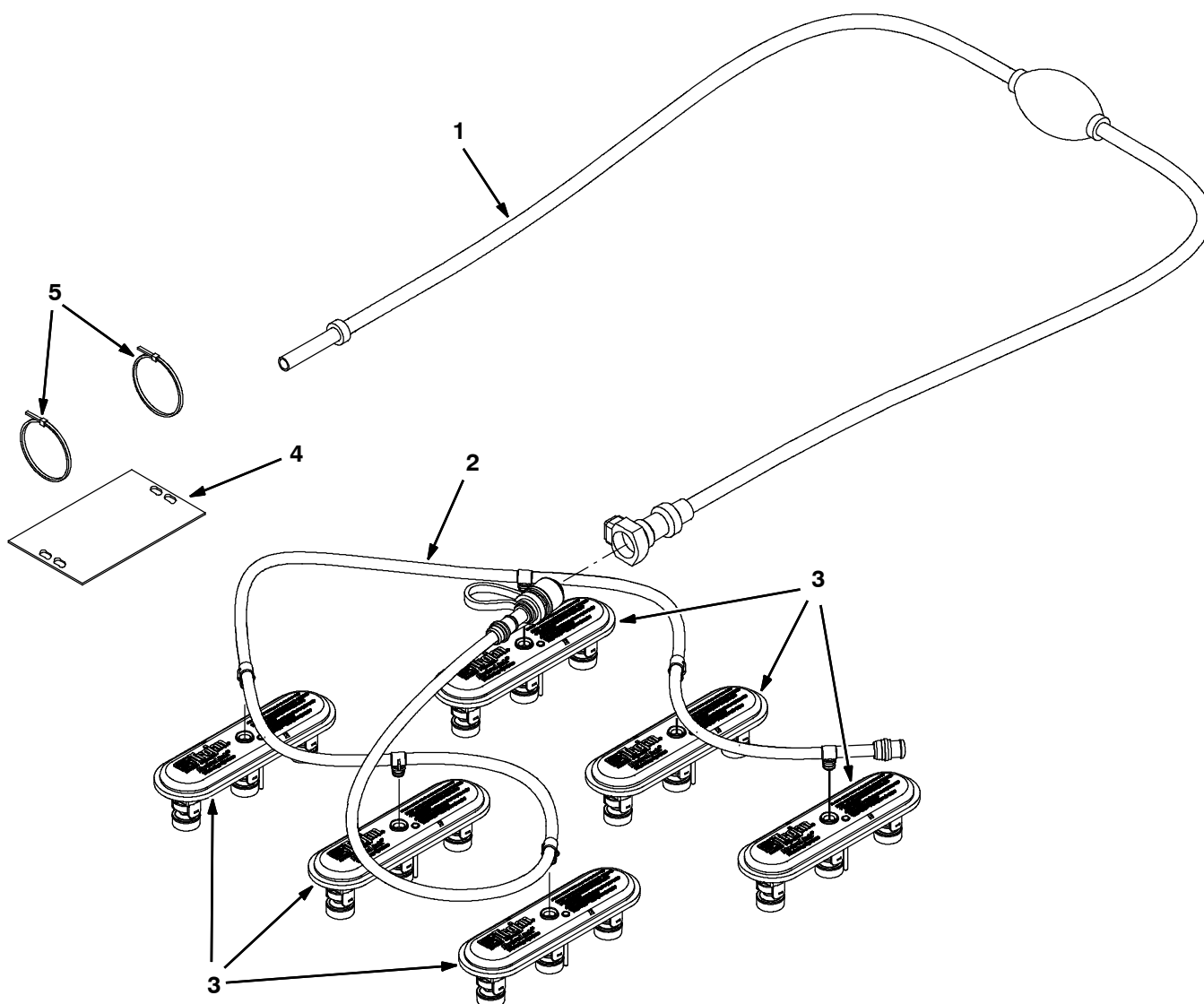
Fig. 44 - Hydrolink® Battery Watering System Kit
