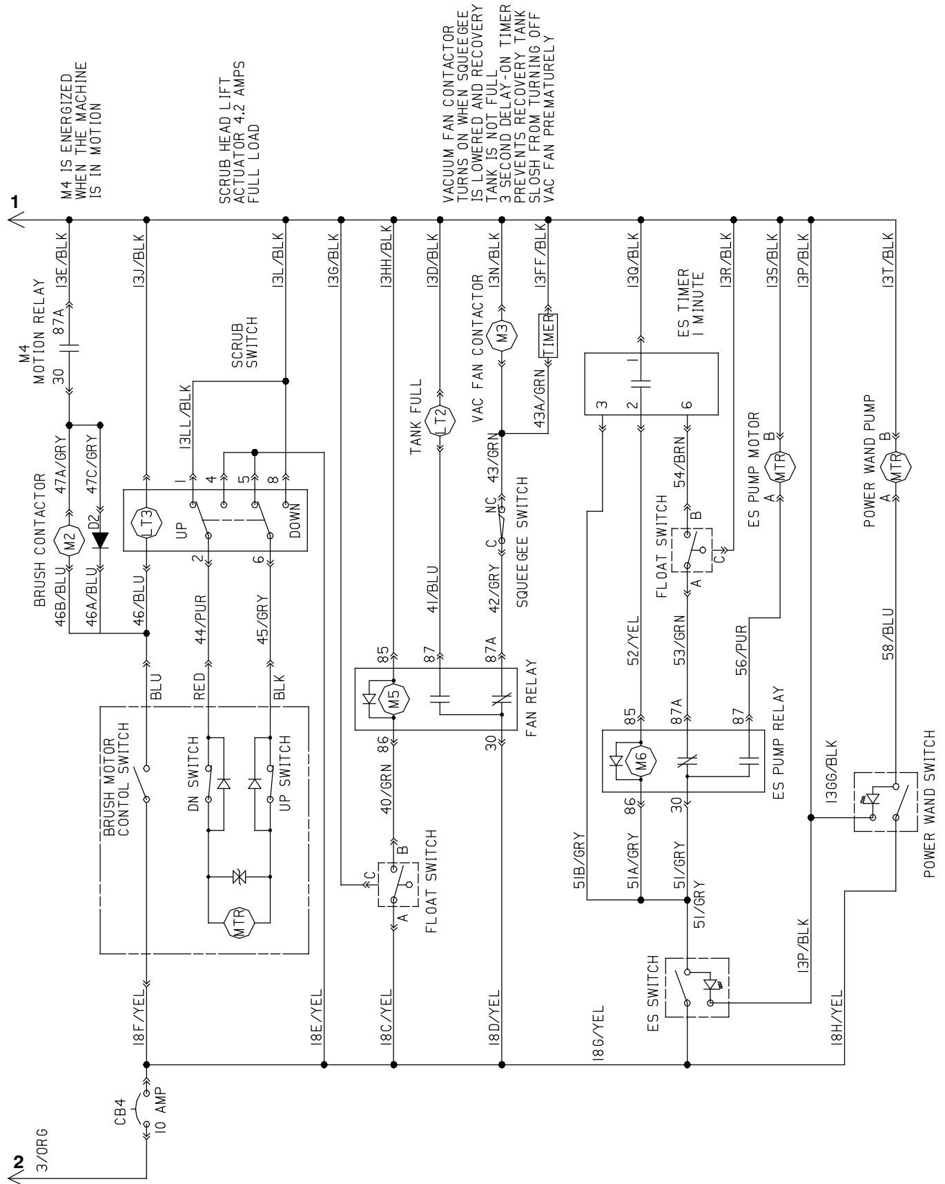
Fig. 35 - Electrical Schematic, Standard &amp; Fast Model
