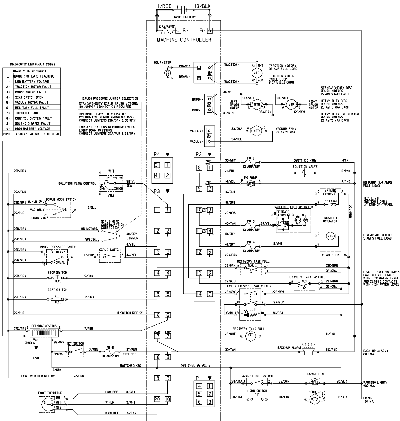
Fig. 27 - Electrical Schematic (00000000-10143032)
