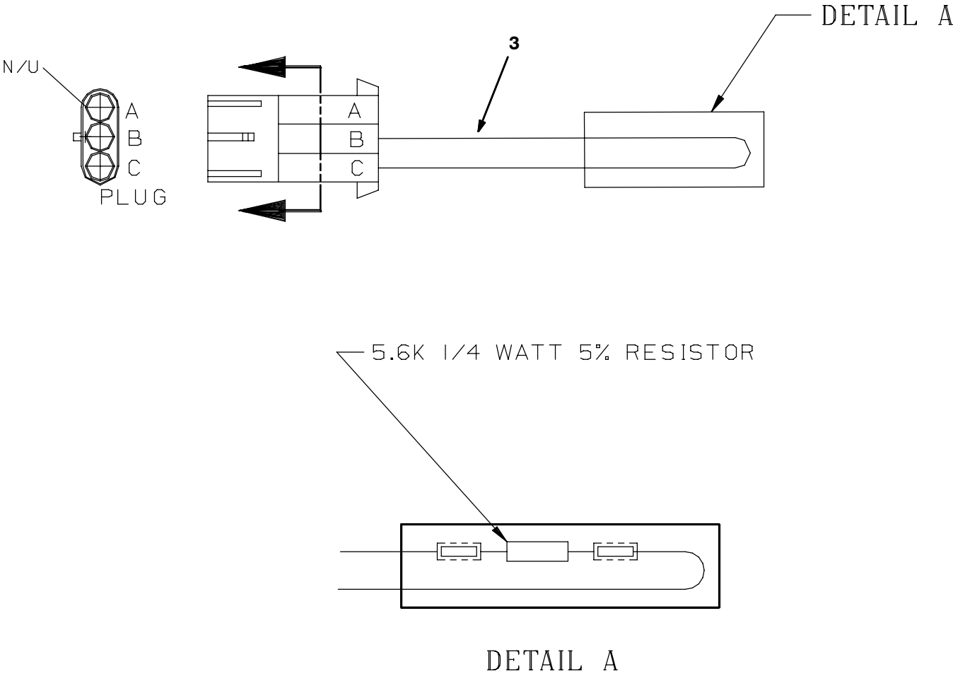
Fig. 9 - FaST Wire Harness Group
