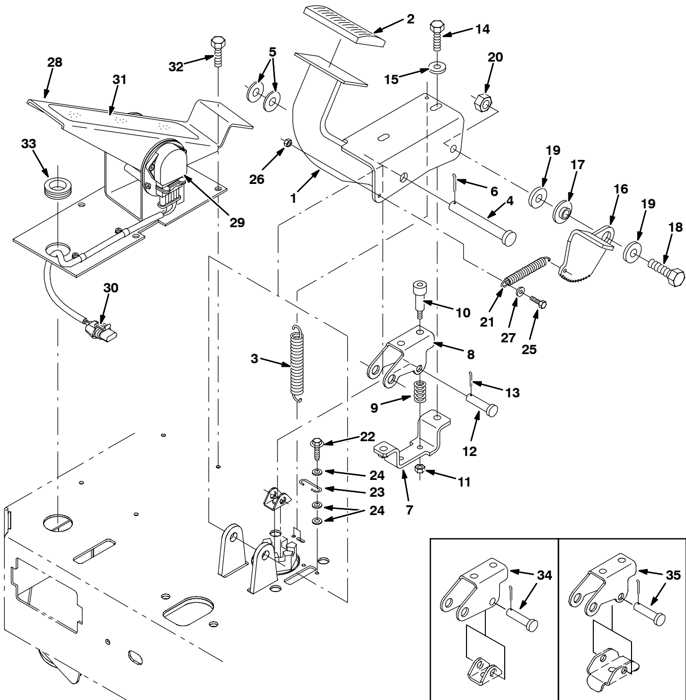
Fig. 12 - Brake Pedal and Directional Pedal Group
