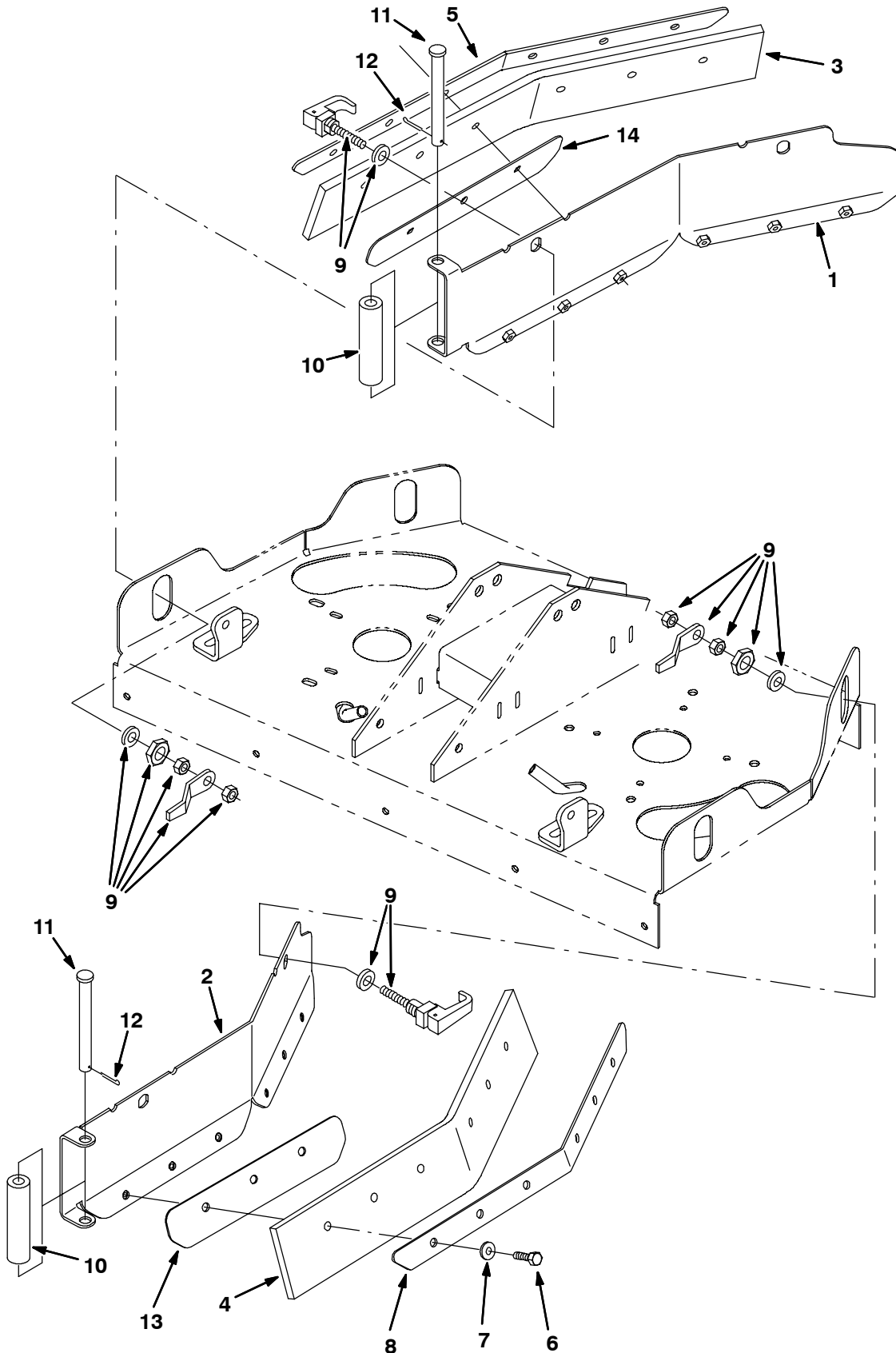
Fig. 17 - Disk Scrub Head Squeegee Group, 700 mm (28 in) (00000000-10214060)
