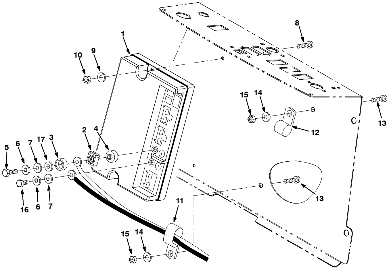
Fig. 8 - Controller Group
