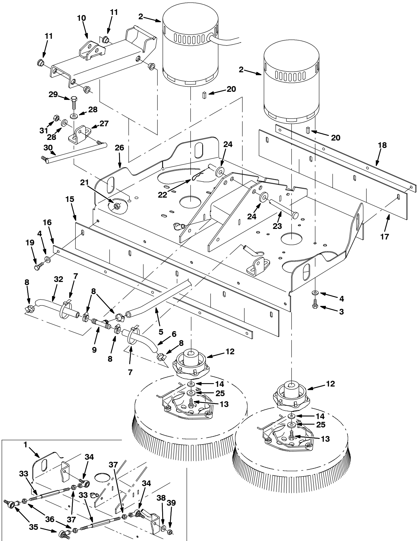
Fig. 15 - Disk Scrub Head Drive Motor Group, 700 mm (28 in) (00000000-10214060)
