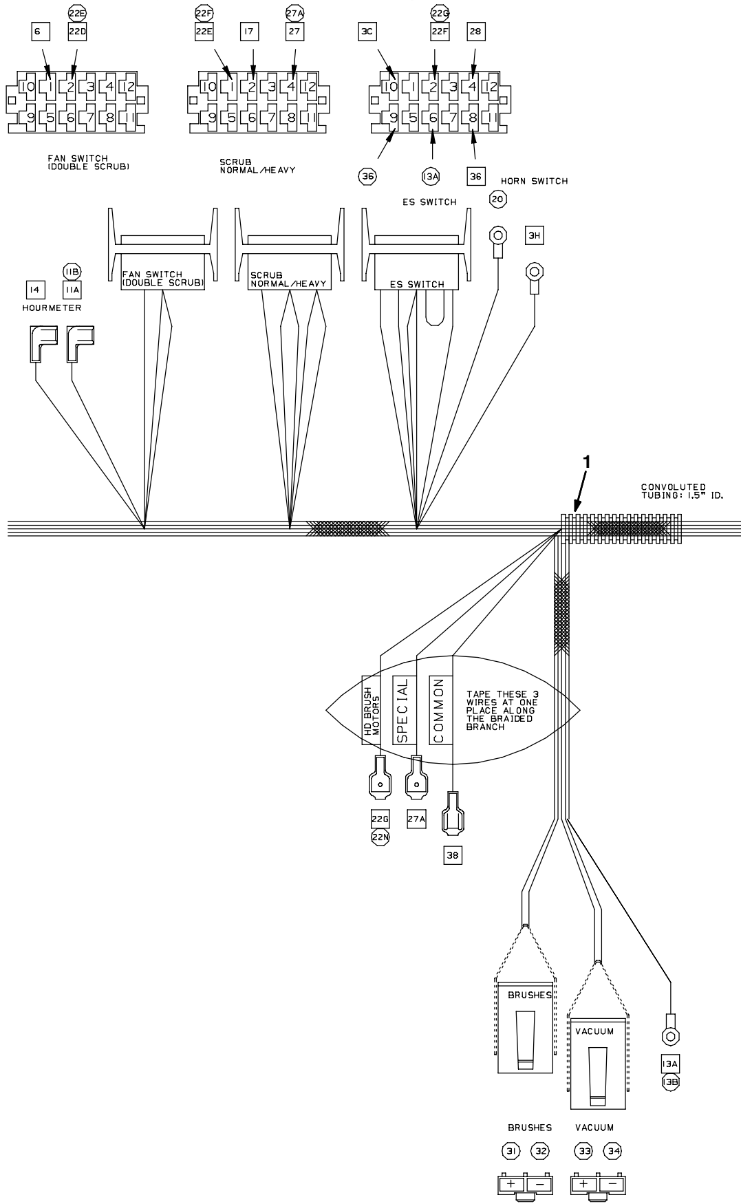
Fig. 30 - Wire Harnesses Group (00000000-10143032)
