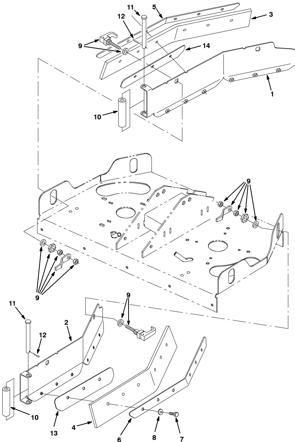
Fig. 18 - Disk Scrub Head Squeegee Group, 800 mm (32 in) (00000000-10214060)
