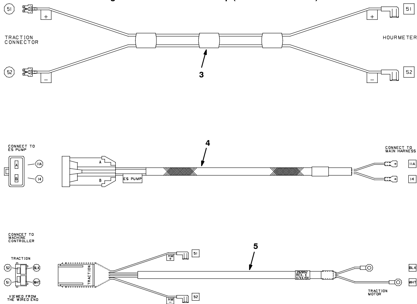
Fig. 31 - Wire Harnesses Group (10143033-10247589)
