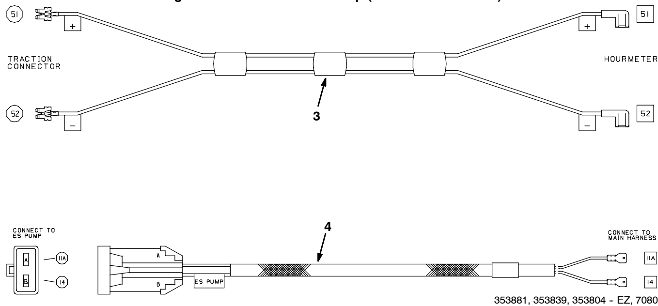
Fig. 30 - Wire Harnesses Group (00000000-10143032)
