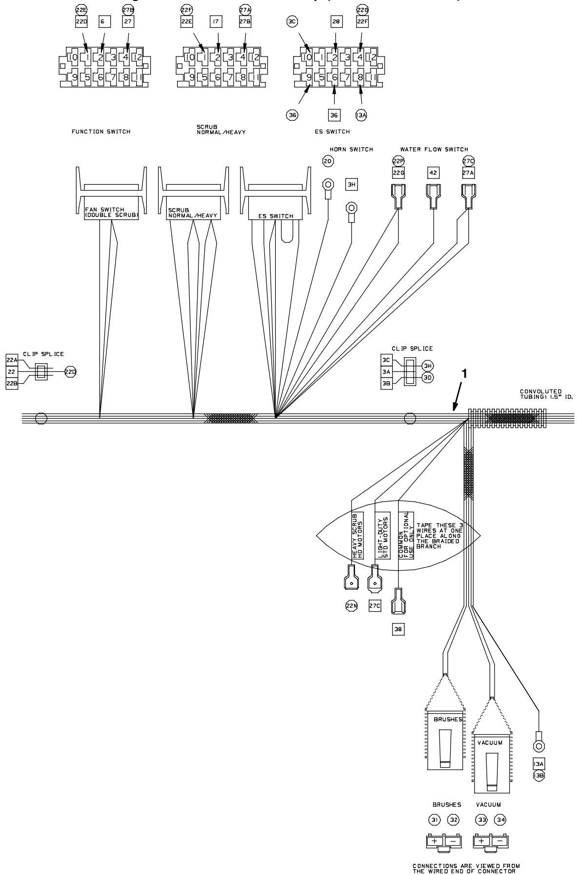
Fig. 31 - Wire Harnesses Group (10143033-10247589)
