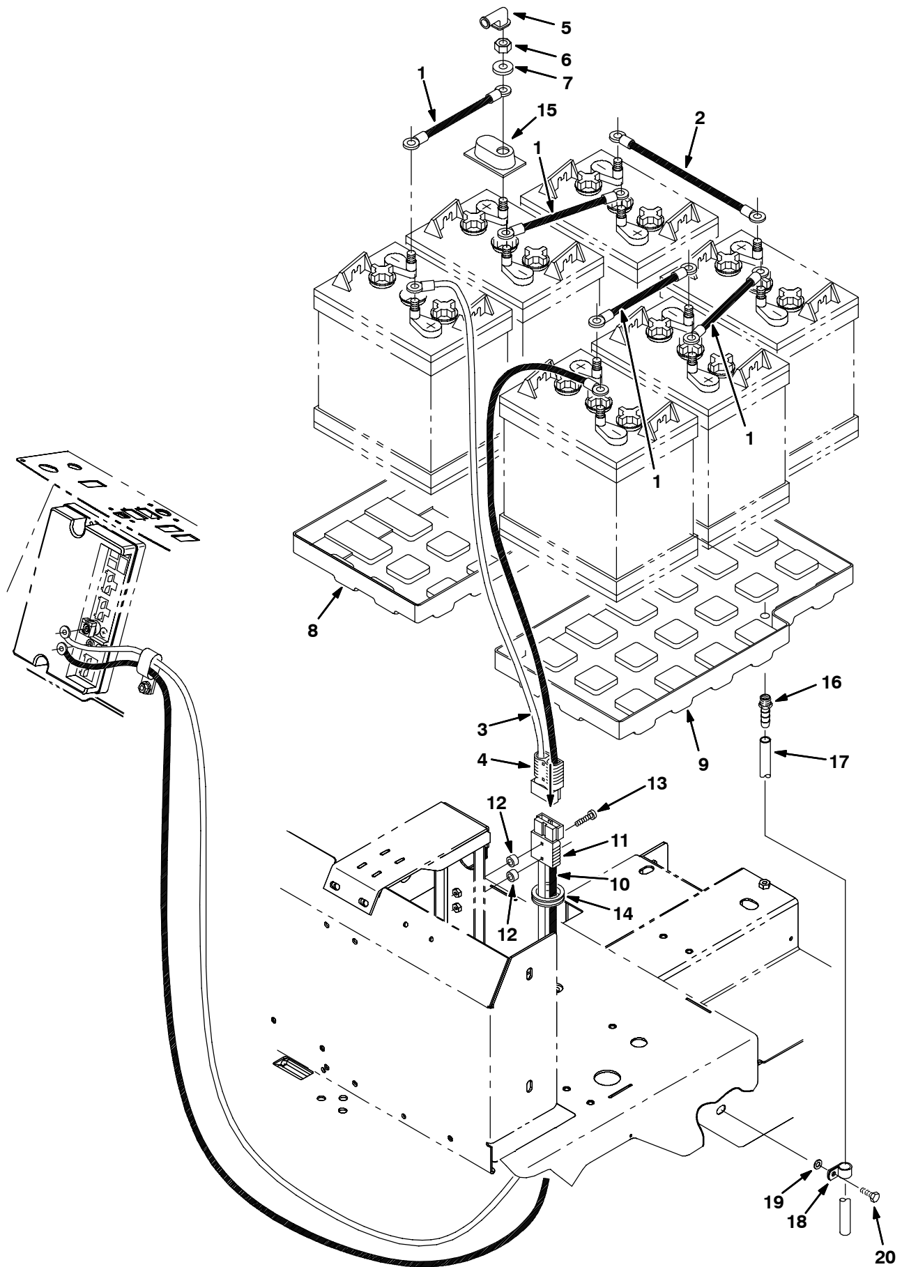
Fig. 23 - Battery Cable Group
