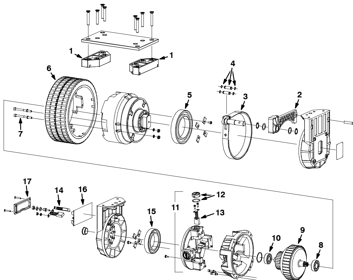
Fig. 6 - Front Wheel Gearbox Breakdown, 374346 (10262872- )
