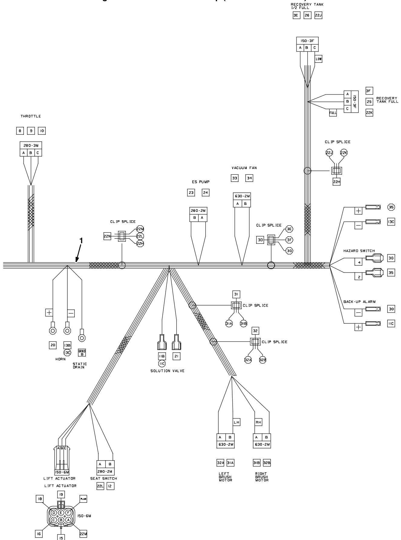
Fig. 30 - Wire Harness Group (00000000-10143032)
