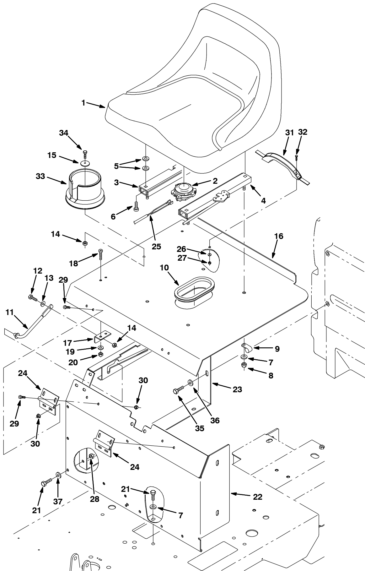
Fig. 5 - Seat Group
