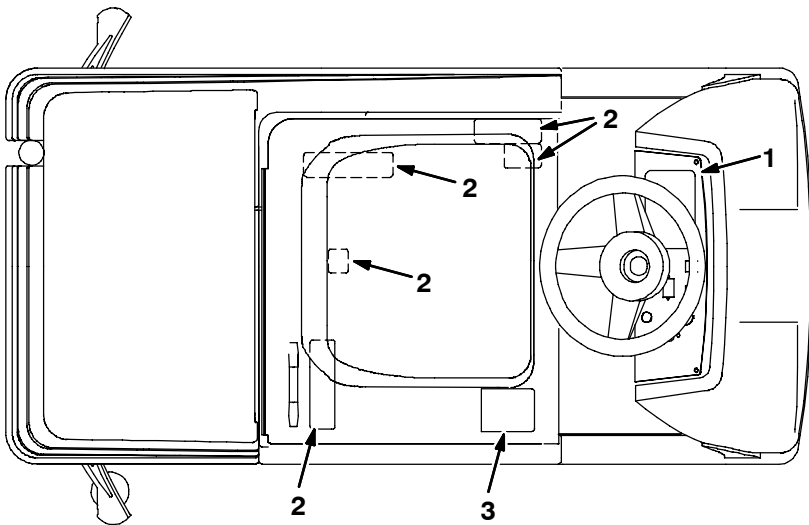
Fig. 33 - Label Group
