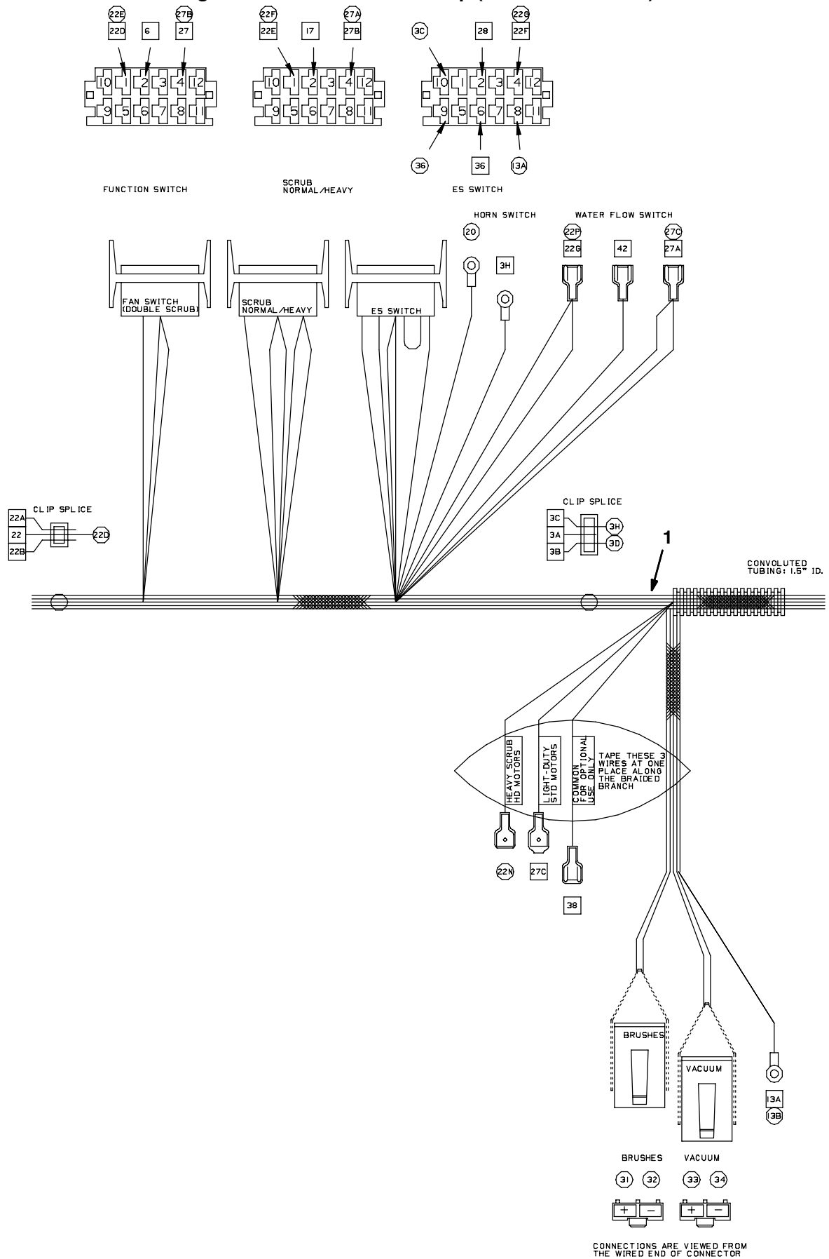
Fig. 32 - Wire Harnesses Group (10247590- )
