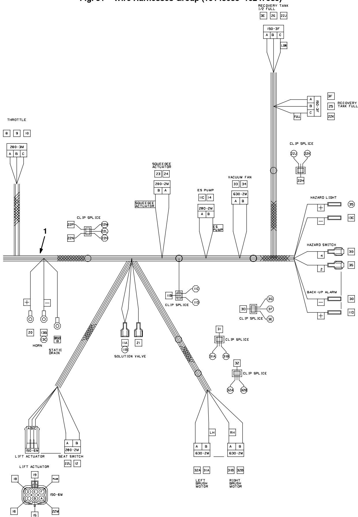
Fig. 31 - Wire Harness Group (10143033-10247589)
