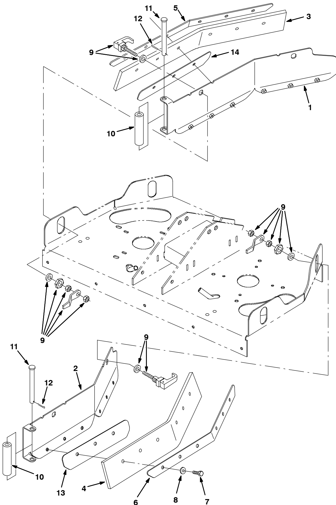
Fig. 14 - Heavy Duty Disk Scrub Head Squeegee Group, 700 mm (28 in) (00000000-10214060)
