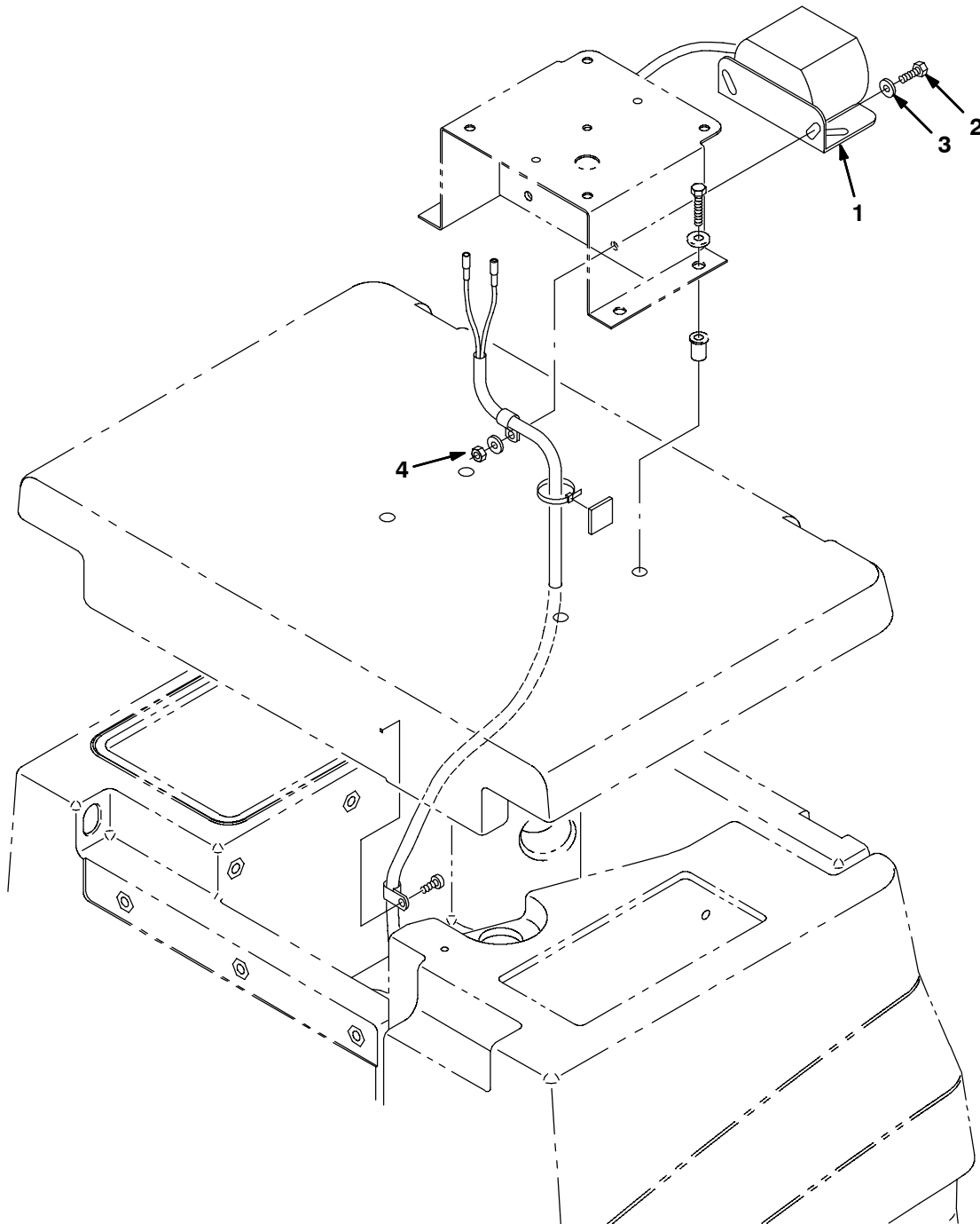
Fig. 30 - Backup Alarm Kit W/O Bracket
