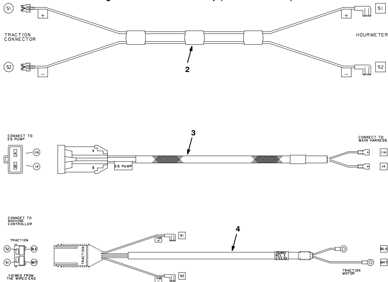
Fig. 32 - Wire Harnesses Group (10247590- )
