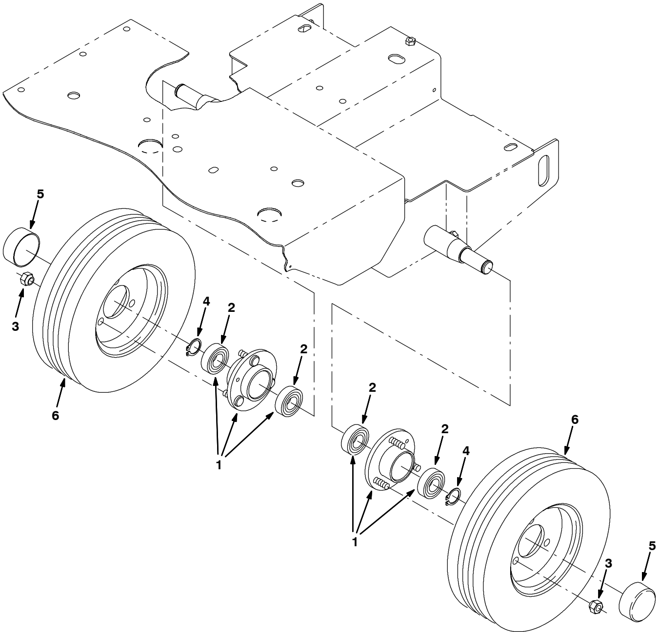
Fig. 13 - Rear Wheel Group
