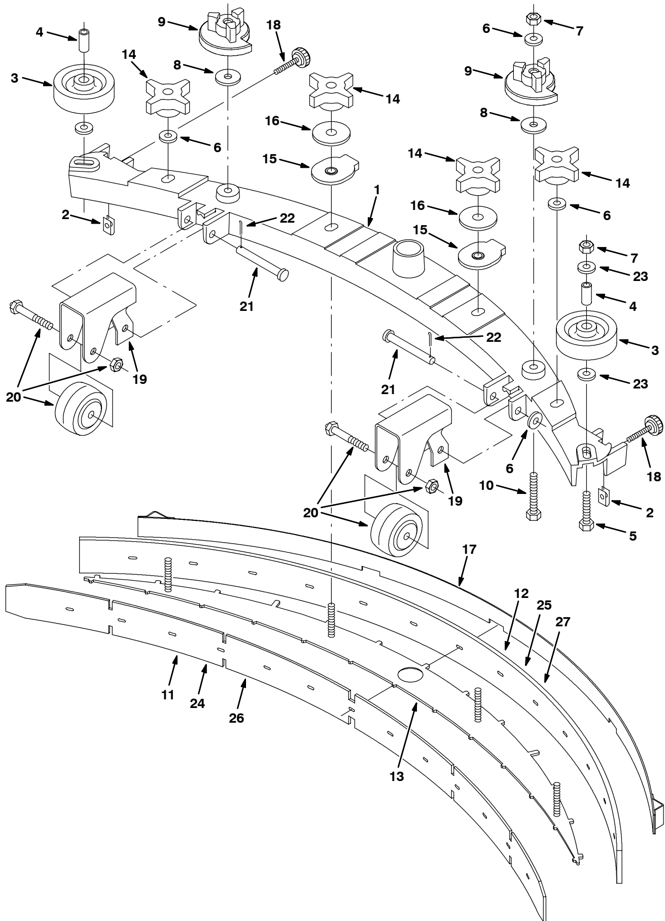
Fig. 26 - Rear Squeegee Group, 800 mm (32 in)
