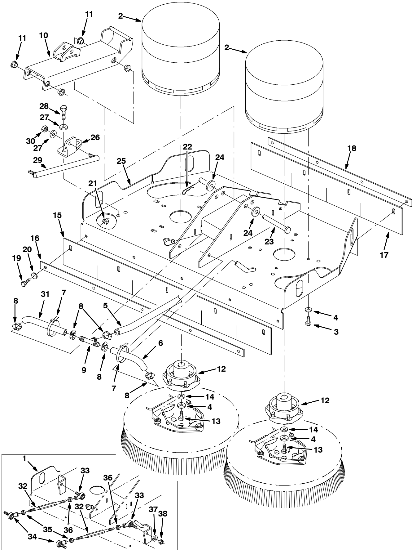
Fig. 16 - Disk Scrub Head Drive Motor Group, 800 mm (32 in) (00000000-10214060)
