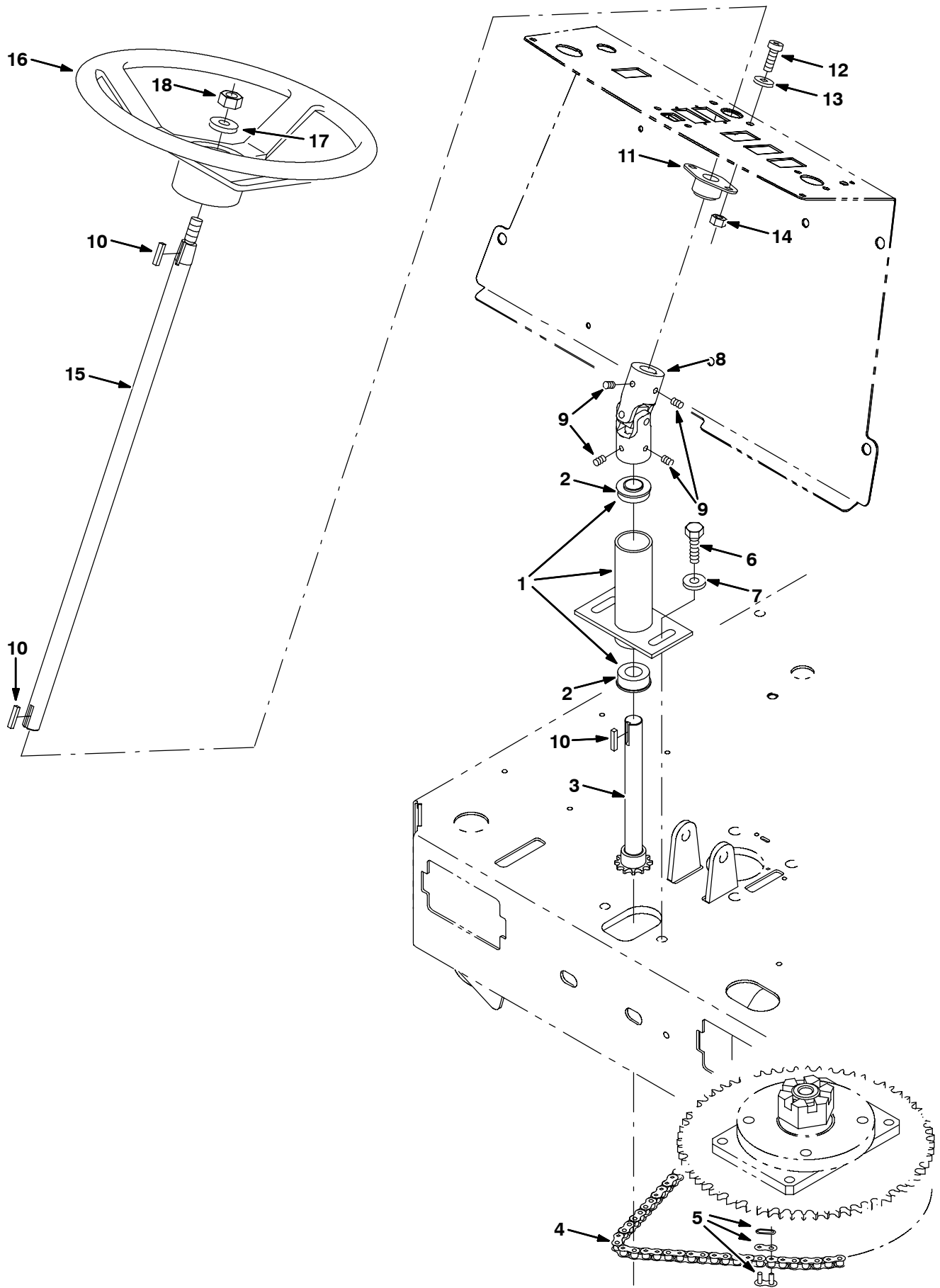
Fig. 6 - Steering Group
