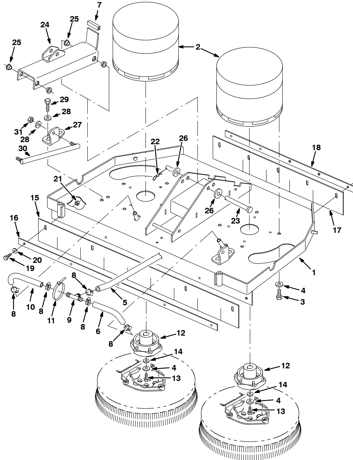
Fig. 17 - Disk Scrub Head Drive Motor Group, 800 mm (32 in) (10214061 - )
