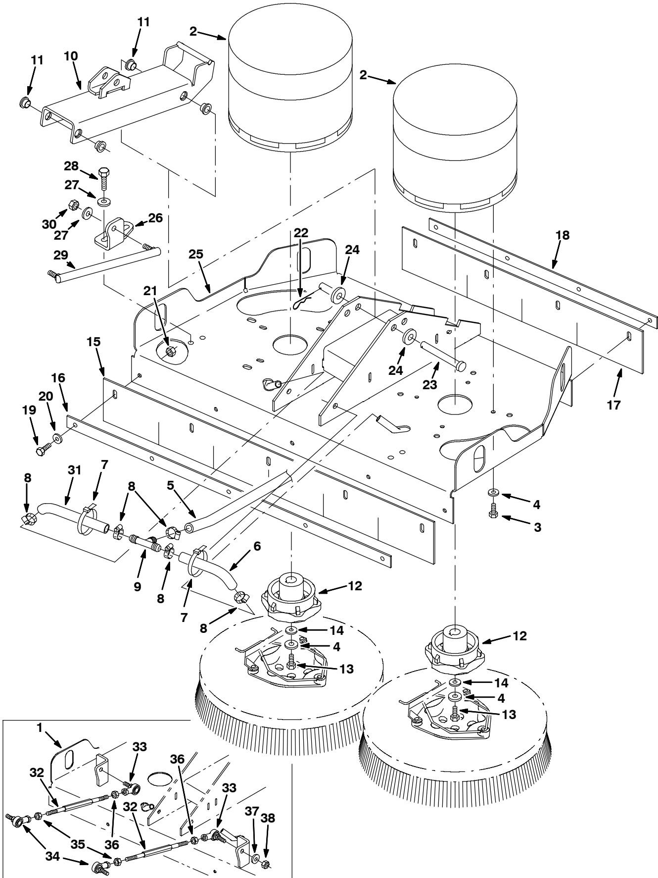
Fig. 12 - Heavy Duty Disk Scrub Head Drive Motor Group, 700 mm (28 in) (00000000-10214060)
