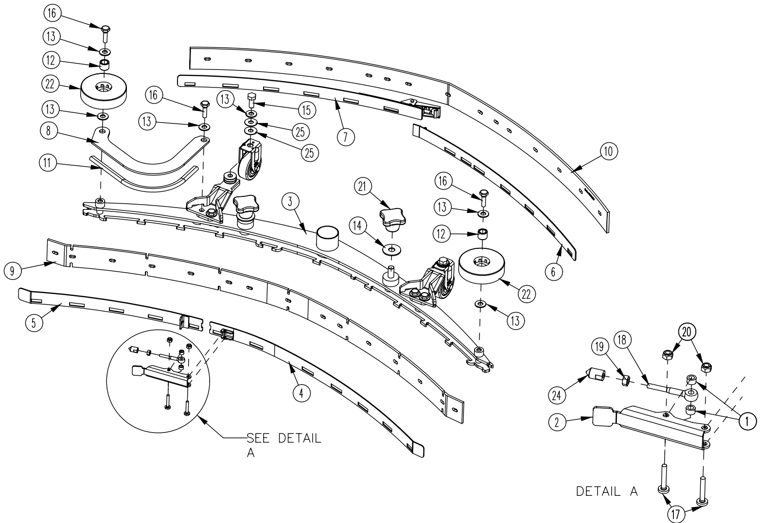
BILL OF MATERIAL - 172270
