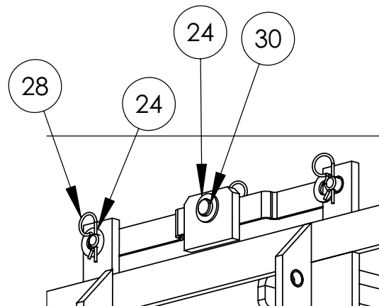
BOTTOM-RIGHT-REAR VIEW
