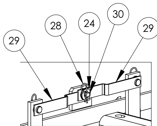
TOP-RIGHT-FRONT VIEW
