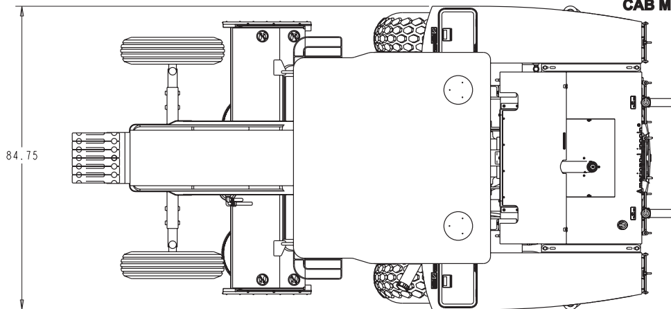
CAB MODEL (TOP VIEW)
