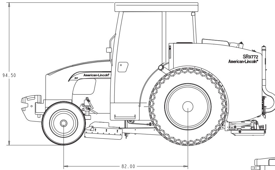
CAB MODEL (SIDE VIEW)
