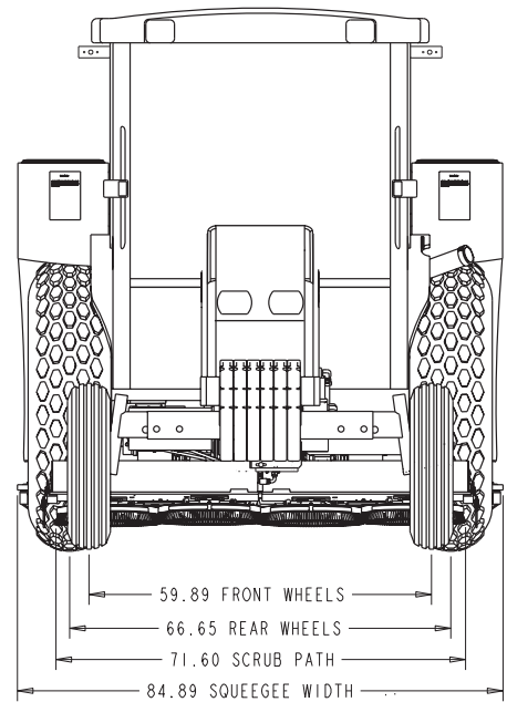
CAB MODEL (REAR VIEW)
