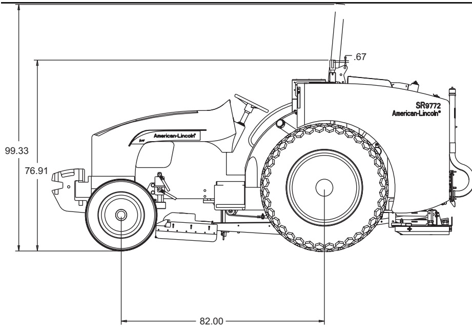
PLATFORM MODEL (SIDE VIEW)
