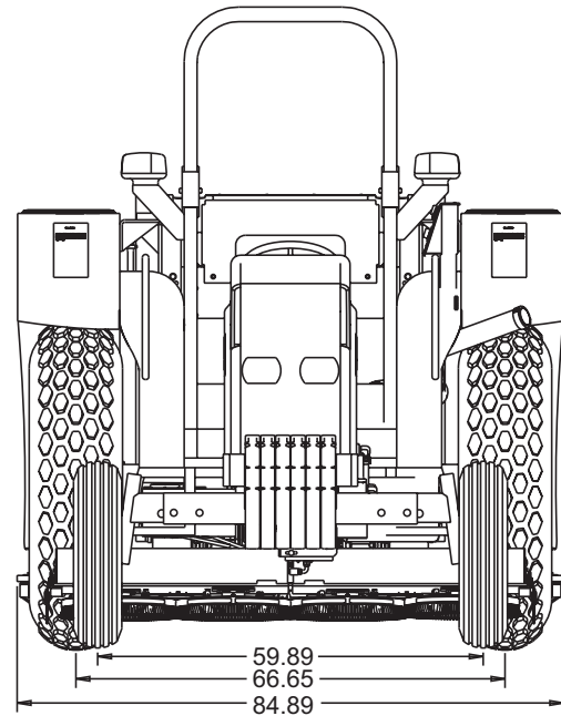
PLATFORM MODEL (REAR VIEW)
