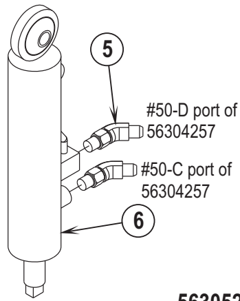
56305244 Squeegee Cylinder Assy
